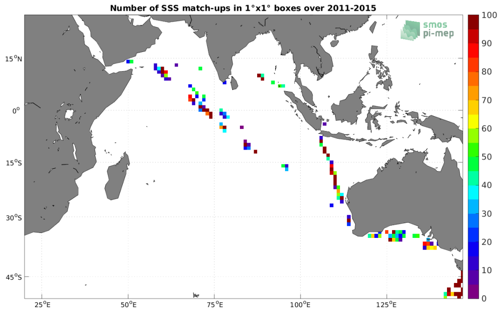
Figure 4: Number of SSS match-ups between TSG (LEGOS-DM) SSS and the Aquarius SSS L2 CAP v5 (JPL) SSS product for the Indian Ocean Pi-MEP region over 1^\circ \times 1^\circ boxes and for the full satellite product period.
