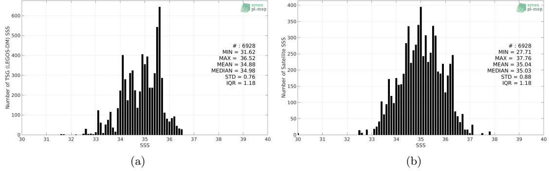
Figure 2: Histograms of SSS from TSG (LEGOS-DM) (a) and Aquarius SSS L2 CAP v5 (JPL) (b) considering all match-up pairs per bins of 0.1 over the Indian Ocean Pi-MEP region and for the full satellite product period.
