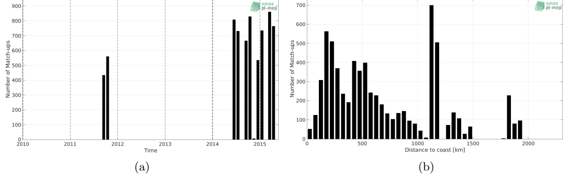
Figure 1: Number of match-ups between TSG (LEGOS-DM) and Aquarius SSS L2 CAP v5 (JPL) SSS as a function of time (a) and as function of the distance to coast (b) over the Indian Ocean Pi-MEP region and for the full satellite product period.
