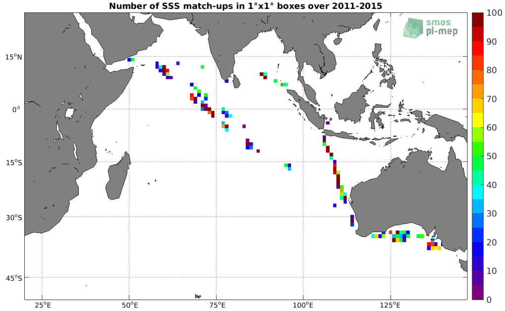
Figure 4: Number of SSS match-ups between TSG (LEGOS-DM) SSS and the Aquarius SSS L2 CAP v5 (JPL) SSS product for the Indian Ocean Pi-MEP region over 1^\circ \times 1^\circ boxes and for the full satellite product period.
