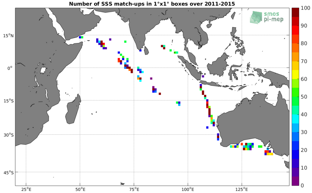
Figure 4: Number of SSS match-ups between TSG-LEGOS-DM SSS and the Aquarius-L2-JPL-V5 SSS product for the Indian Ocean Pi-MEP region over 1^\circ \times 1^\circ boxes and for the full satellite product period.
