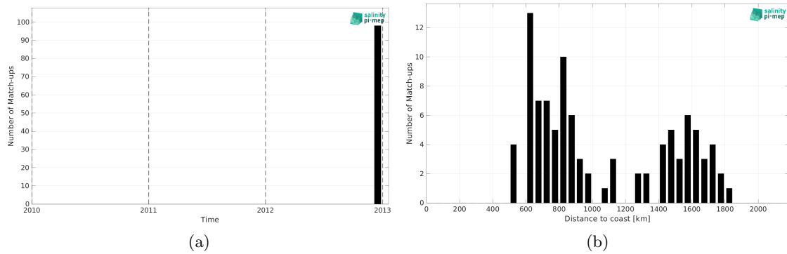
Figure 2: Number of match-ups between TSG (GOSUD-Sailing-ship) and Aquarius SSS L2 CAP v5 (JPL) SSS as a function of time (a) and as function of the distance to coast (b) over the Indian Ocean Pi-MEP region and for the full satellite product period.
