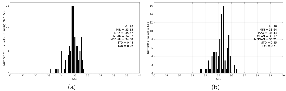
Figure 3: Histograms of SSS from TSG (GOSUD-Sailing-ship) (a) and Aquarius SSS L2 CAP v5 (JPL) (b) considering all match-up pairs per bins of 0.1 over the Indian Ocean Pi-MEP region and for the full satellite product period.
