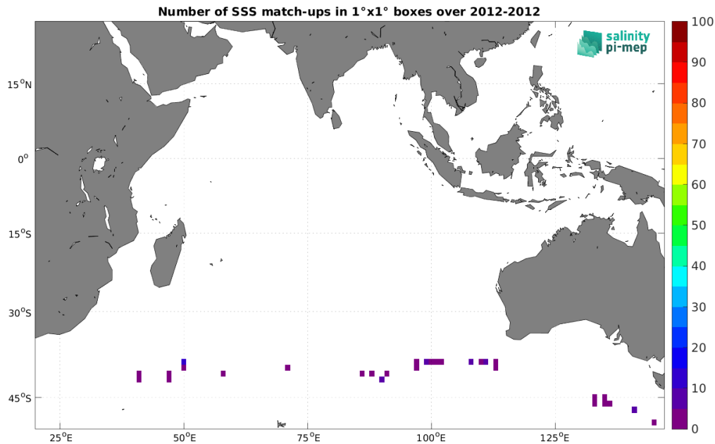
Figure 4: Number of SSS match-ups between TSG (GOSUD-Sailing-ship) SSS and the Aquarius SSS L2 CAP v5 (JPL) SSS product for the Indian Ocean Pi-MEP region over 1^\circ \times 1^\circ boxes and for the full satellite product period.
