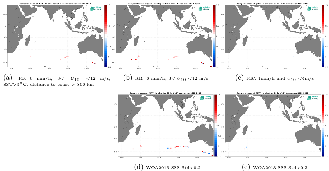
Figure 12: Temporal mean gridded over spatial boxes of size 1^\circ \times 1^\circ of \Delta\text{SSS} (Aquarius SSS L2 CAP v5 (JPL) - TSG (GOSUD-Sailing-ship)) for 5 different subdatasets corresponding to: RR=0 mm/h, 3 < U_{10} < 12 m/s, SST > 5°C, distance to coast > 800 km (a), RR=0 mm/h, 3 < U_{10} < 12 m/s (b), RR > 1mm/h and U_{10} < 4 m/s (c), WOA2013 SSS Std < 0.2 (d), WOA2013 SSS Std > 0.2 (e).
