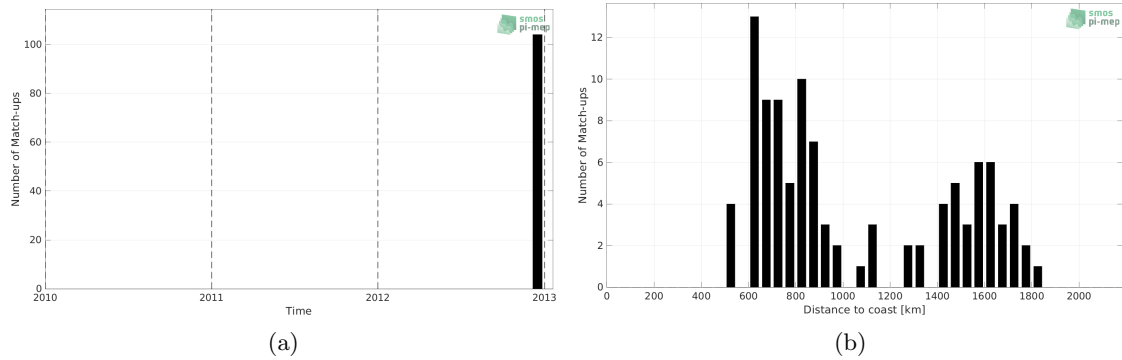
Figure 1: Number of match-ups between TSG (GOSUD-Sailing-ship) and Aquarius SSS L2 CAP v5 (JPL) SSS as a function of time (a) and as function of the distance to coast (b) over the Indian Ocean Pi-MEP region and for the full satellite product period.
