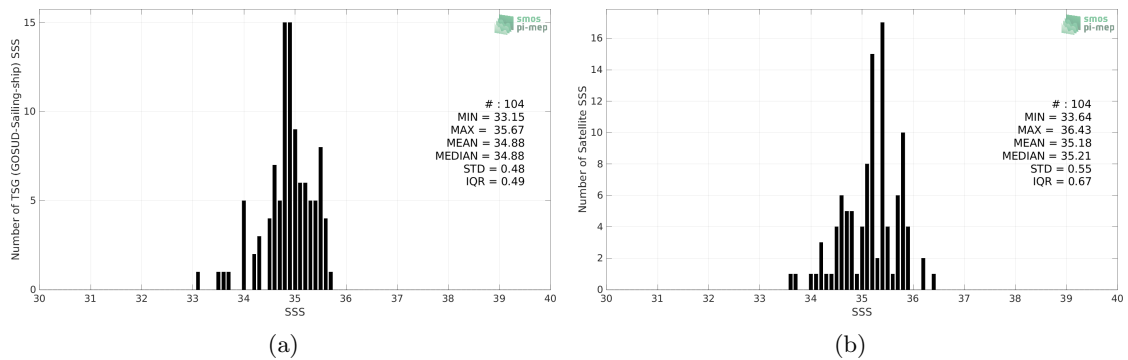
Figure 2: Histograms of SSS from TSG (GOSUD-Sailing-ship) (a) and Aquarius SSS L2 CAP v5 (JPL) (b) considering all match-up pairs per bins of 0.1 over the Indian Ocean Pi-MEP region and for the full satellite product period.
