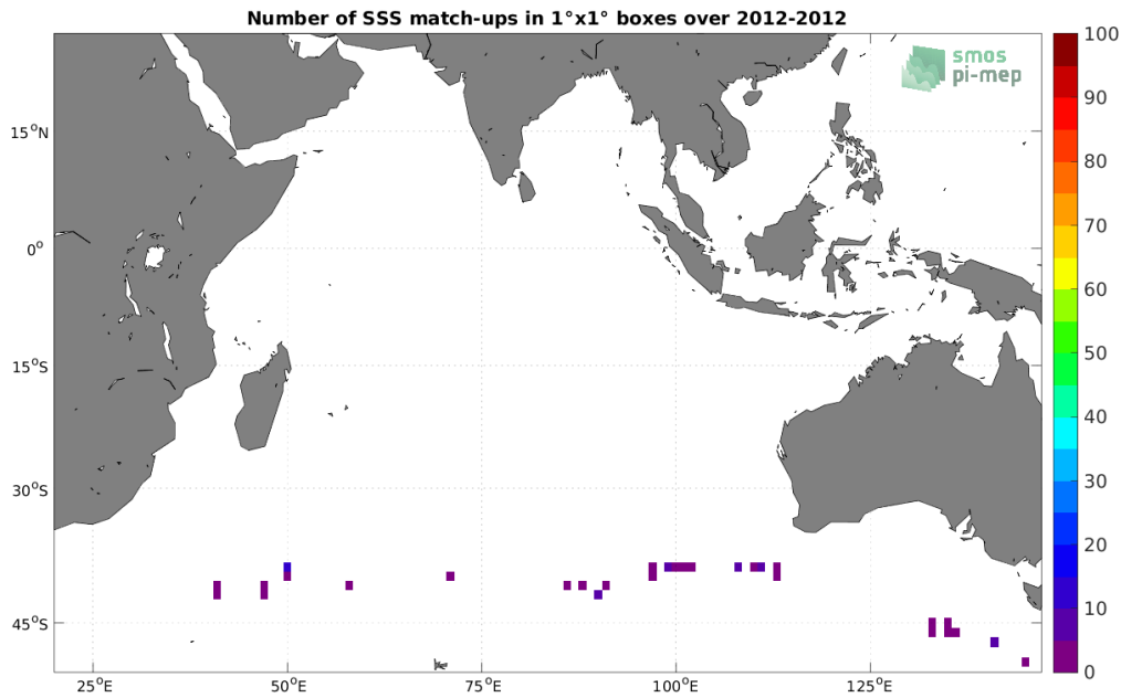
Figure 4: Number of SSS match-ups between TSG (GOSUD-Sailing-ship) SSS and the Aquarius SSS L2 CAP v5 (JPL) SSS product for the Indian Ocean Pi-MEP region over 1^\circ \times 1^\circ boxes and for the full satellite product period.
