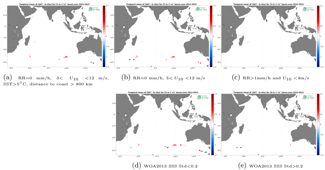
Figure 12: Temporal mean gridded over spatial boxes of size 1^\circ \times 1^\circ of \Delta SSS (Aquarius SSS L2 CAP v5 (JPL) - TSG (GOSUD-Sailing-ship)) for 5 different subdatasets corresponding to: RR=0 mm/h, 3 < U_{10} < 12 m/s, SST > 5°C, distance to coast > 800 km (a), RR=0 mm/h, 3 < U_{10} < 12 m/s (b), RR > 1mm/h and U_{10} < 4 m/s (c), WOA2013 SSS Std < 0.2 (d), WOA2013 SSS Std > 0.2 (e).
