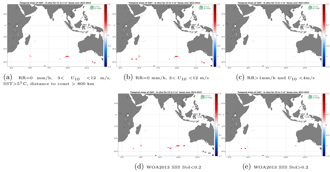
Figure 12: Temporal mean gridded over spatial boxes of size 1^\circ \times 1^\circ of \Delta SSS (Aquarius-L2-JPL-V5 - TSG-GOSUD-Sailing-ship) for 5 different subdatasets corresponding to: RR=0 mm/h, 3 < U_{10} < 12 m/s, SST > 5^\circ\text{C} , distance to coast > 800 km (a), RR=0 mm/h, 3 < U_{10} < 12 m/s (b), RR > 1 mm/h and U_{10} < 4 m/s (c), WOA2013 SSS Std < 0.2 (d), WOA2013 SSS Std > 0.2 (e).
