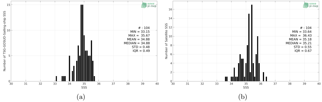
Figure 2: Histograms of SSS from TSG-GOSUD-Sailing-ship (a) and Aquarius-L2-JPL-V5 (b) considering all match-up pairs per bins of 0.1 over the Indian Ocean Pi-MEP region and for the full satellite product period.
