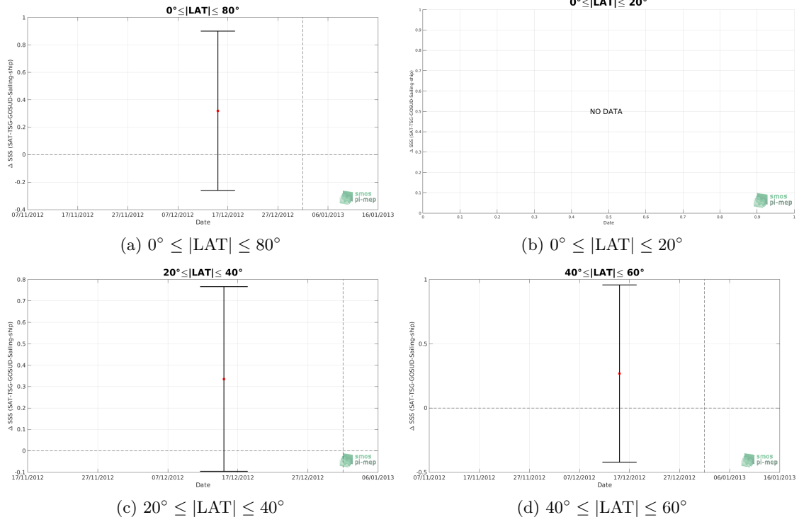
Figure 10: Monthly median (red curves) of \Delta\text{SSS} (Satellite - TSG-GOSUD-Sailing-ship) and \pm 1 Std (black vertical thick bars) as function of time for all the collected Pi-MEP match-up pairs estimated over the Indian Ocean Pi-MEP region and for the full satellite product period are shown for different latitude bands: (a) 80°S-80°N, (b) 20°S-20°N, (c) 40°S-20°S and 20°N-40°N and (d) 60°S-40°S and 40°N-60°N.
