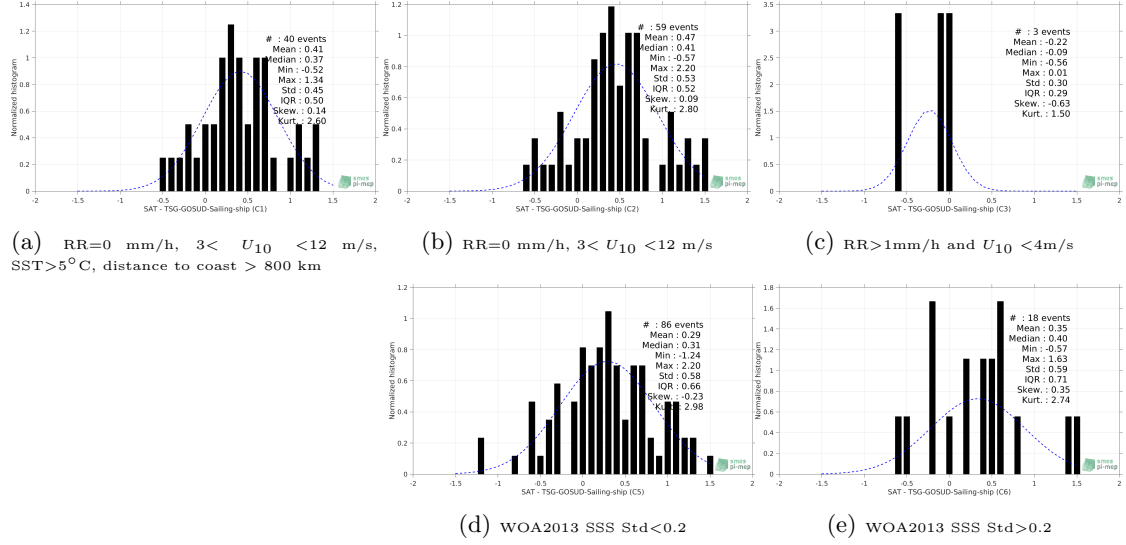
Figure 13: Normalized histogram of \Delta\text{SSS} (Aquarius-L2-JPL-V5 - TSG-GOSUD-Sailing-ship) for 5 different subdatasets corresponding to: RR=0 mm/h, 3 < U_{10} < 12 m/s, SST >5^{\circ}\text{C} , distance to coast > 800 km (a), RR=0 mm/h, 3 < U_{10} < 12 m/s (b), RR>1\text{mm/h} and U_{10} < 4\text{m/s} (c), WOA2013 SSS Std <0.2 (d), WOA2013 SSS Std >0.2 (e).
