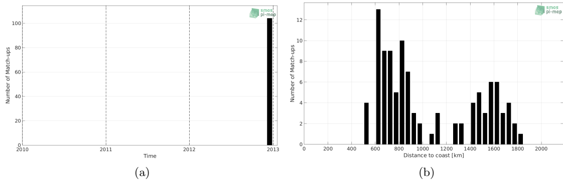
Figure 1: Number of match-ups between TSG-GOSUD-Sailing-ship and Aquarius-L2-JPL-V5 SSS as a function of time (a) and as function of the distance to coast (b) over the Indian Ocean Pi-MEP region and for the full satellite product period.
