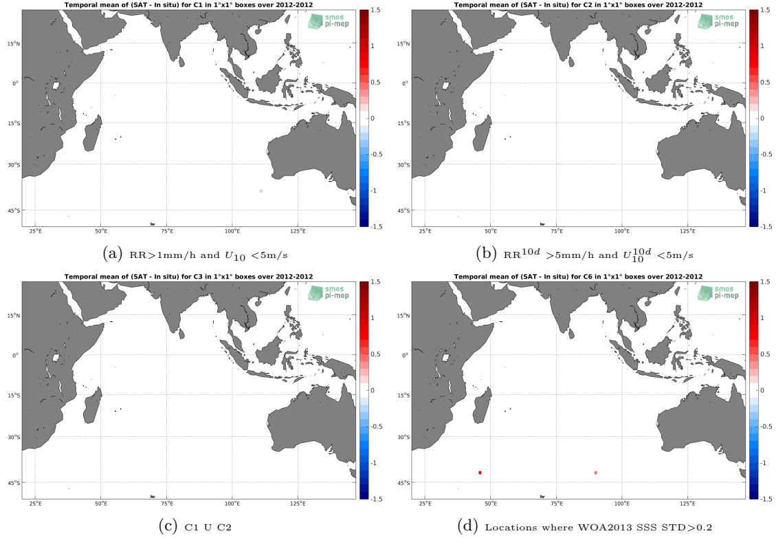
Figure 12: Temporal mean gridded over spatial boxes of size 1^\circ \times 1^\circ of \Delta SSS (Aquarius-L2-JPL-V5 - TSG-GOSUD-Sailing-ship) for 4 different subdatasets corresponding to: RR > 1\text{mm/h} and U_{10} < 5\text{m/s} (a), RR^{10d} > 5\text{mm/h} and U_{10}^{10d} < 5\text{m/s} (b), C1 U C2 (c), Locations where WOA2013 SSS STD > 0.2 (d).
