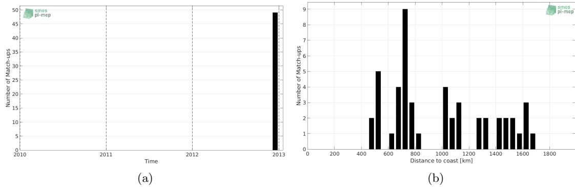
Figure 1: Number of match-ups between TSG-GOSUD-Sailing-ship and Aquarius-L2-JPL-V5 SSS as a function of time (a) and as function of the distance to coast (b) over the Indian Ocean Pi-MEP region and for the full satellite product period.
