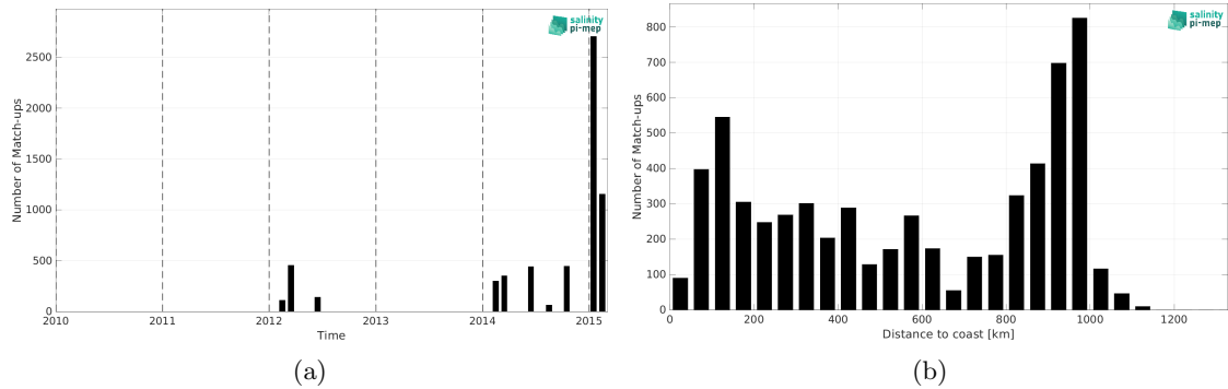
Figure 2: Number of match-ups between TSG (GOSUD-Research-vessel) and Aquarius SSS L2 CAP v5 (JPL) SSS as a function of time (a) and as function of the distance to coast (b) over the Indian Ocean Pi-MEP region and for the full satellite product period.
