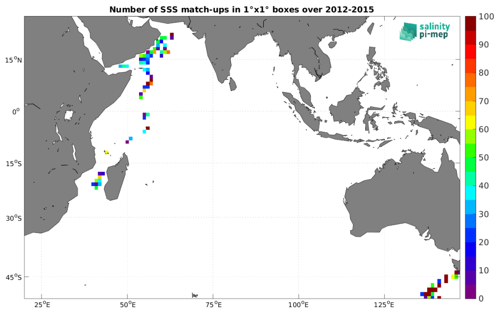
Figure 5: Number of SSS match-ups between TSG (GOSUD-Research-vessel) SSS and the Aquarius SSS L2 CAP v5 (JPL) SSS product for the Indian Ocean Pi-MEP region over 1^\circ \times 1^\circ boxes and for the full satellite product period.
