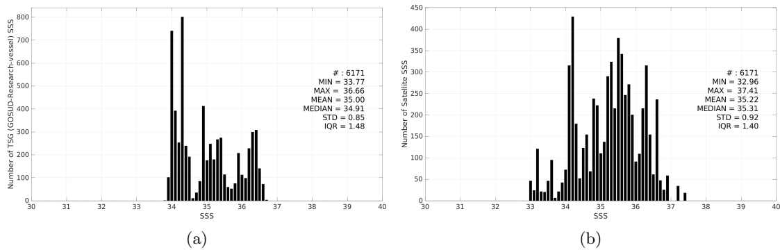
Figure 3: Histograms of SSS from TSG (GOSUD-Research-vessel) (a) and Aquarius SSS L2 CAP v5 (JPL) (b) considering all match-up pairs per bins of 0.1 over the Indian Ocean Pi-MEP region and for the full satellite product period.
