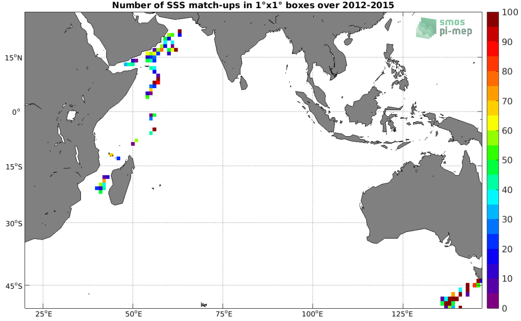
Figure 4: Number of SSS match-ups between TSG (GOSUD-Research-vessel) SSS and the Aquarius SSS L2 CAP v5 (JPL) SSS product for the Indian Ocean Pi-MEP region over 1^\circ \times 1^\circ boxes and for the full satellite product period.
