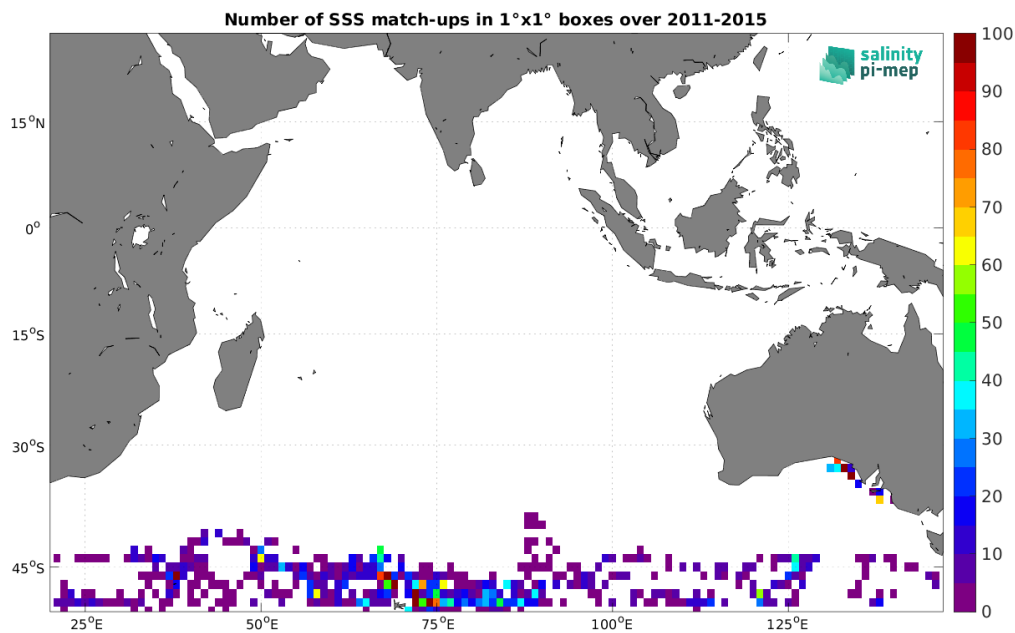
Figure 4: Number of SSS match-ups between Marine mammals SSS and the Aquarius SSS L2 CAP v5 (JPL) SSS product for the Indian Ocean Pi-MEP region over 1^\circ \times 1^\circ boxes and for the full satellite product period.
