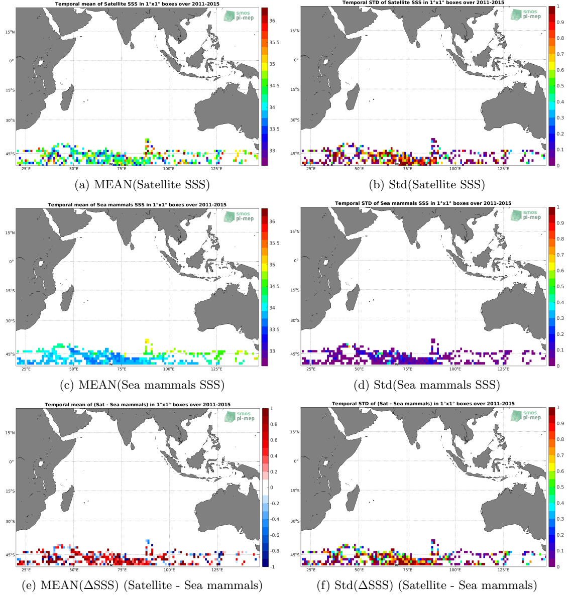
Figure 6: Temporal mean (left) and Std (right) of SSS from Aquarius SSS L2 CAP v5 (JPL) (top), Sea mammals (middle), and of \Delta SSS (Satellite - Sea mammals). Only match-up pairs are used to generate these maps.
