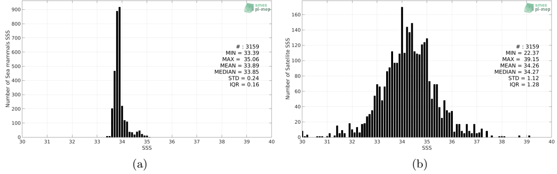
Figure 2: Histograms of SSS from Sea mammals (a) and Aquarius SSS L2 CAP v5 (JPL) (b) considering all match-up pairs per bins of 0.1 over the Indian Ocean Pi-MEP region and for the full satellite product period.
