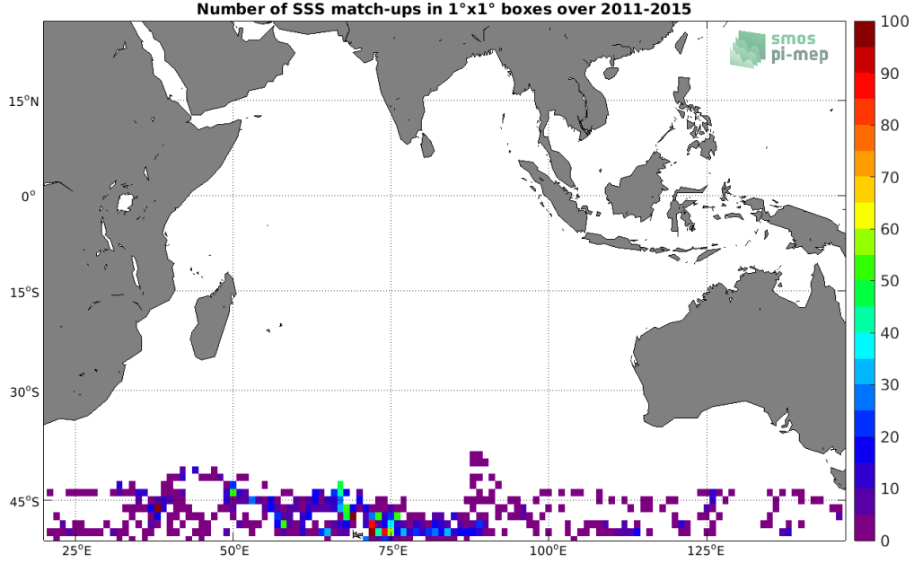
Figure 4: Number of SSS match-ups between Sea mammals SSS and the Aquarius SSS L2 CAP v5 (JPL) SSS product for the Indian Ocean Pi-MEP region over 1^\circ \times 1^\circ boxes and for the full satellite product period.
