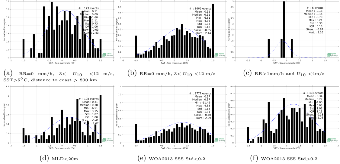
Figure 13: Normalized histogram of \Delta SSS (Aquarius SSS L2 CAP v5 (JPL) - Sea mammals) for 6 different subdatasets corresponding to: RR=0 mm/h, 3 < U_{10} < 12 m/s, SST>5°C, distance to coast > 800 km (a), RR=0 mm/h, 3 < U_{10} < 12 m/s (b), RR>1mm/h and U_{10} < 4 m/s (c), MLD<20m (d), WOA2013 SSS Std<0.2 (e), WOA2013 SSS Std>0.2 (f).
