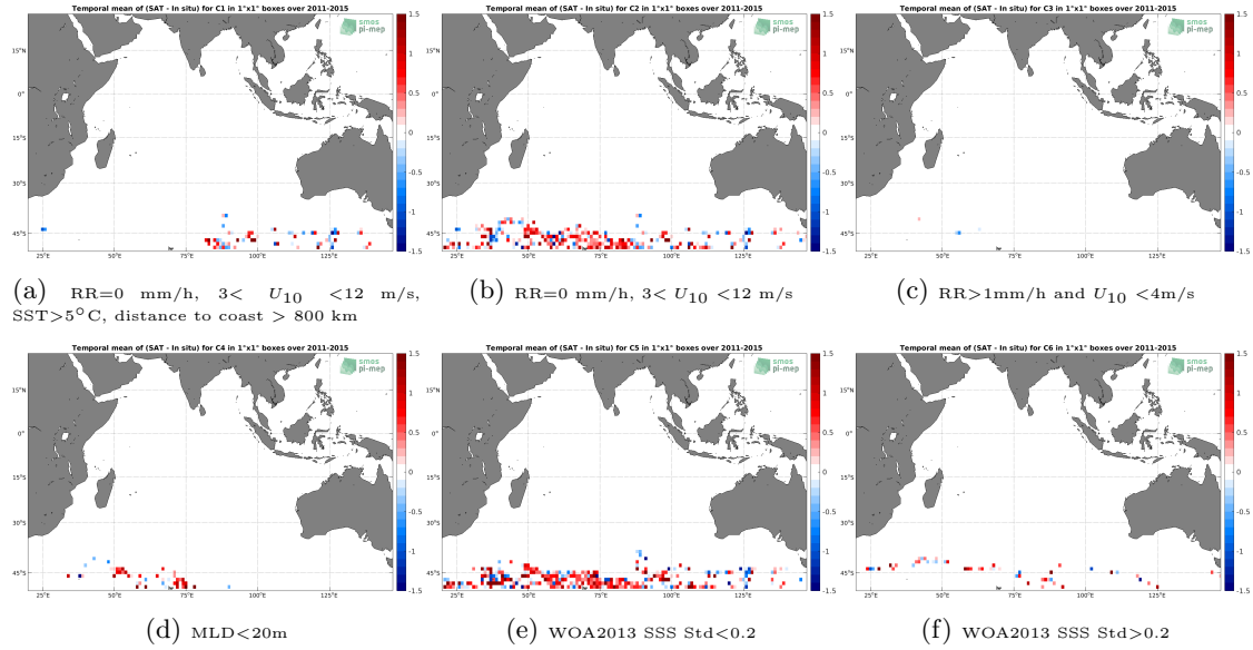
Figure 12: Temporal mean gridded over spatial boxes of size 1^{\circ}\times 1^{\circ} of \Delta\text{SSS} (Aquarius SSS L2 CAP v5 (JPL) - Sea mammals) for 6 different subdatasets corresponding to: \text{RR}=0 mm/h, 3 < U_{10} < 12 m/s, \text{SST} > 5^{\circ}\text{C} , distance to coast > 800 km (a), \text{RR}=0 mm/h, 3 < U_{10} < 12 m/s (b), \text{RR} > 1\text{mm/h} and U_{10} < 4\text{m/s} (c), \text{MLD} < 20\text{m} (d), \text{WOA2013 SSS Std} < 0.2 (e), \text{WOA2013 SSS Std} > 0.2 (f).
