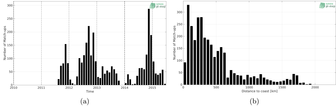
Figure 1: Number of match-ups between Sea mammals and Aquarius SSS L2 CAP v5 (JPL) SSS as a function of time (a) and as function of the distance to coast (b) over the Indian Ocean Pi-MEP region and for the full satellite product period.
