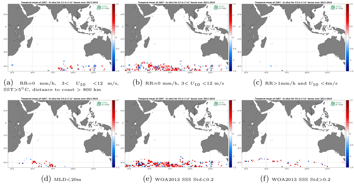
Figure 12: Temporal mean gridded over spatial boxes of size 1^{\circ}\times 1^{\circ} of \Delta\text{SSS} (Aquarius-L2-JPL-V5 - Sea mammals) for 6 different subdatasets corresponding to: \text{RR}=0 mm/h, 3 < U_{10} < 12 m/s, \text{SST} > 5^{\circ}\text{C} , distance to coast > 800 km (a), \text{RR}=0 mm/h, 3 < U_{10} < 12 m/s (b), \text{RR} > 1\text{mm/h} and U_{10} < 4\text{m/s} (c), \text{MLD} < 20\text{m} (d), WOA2013 SSS Std < 0.2 (e), WOA2013 SSS Std > 0.2 (f).
