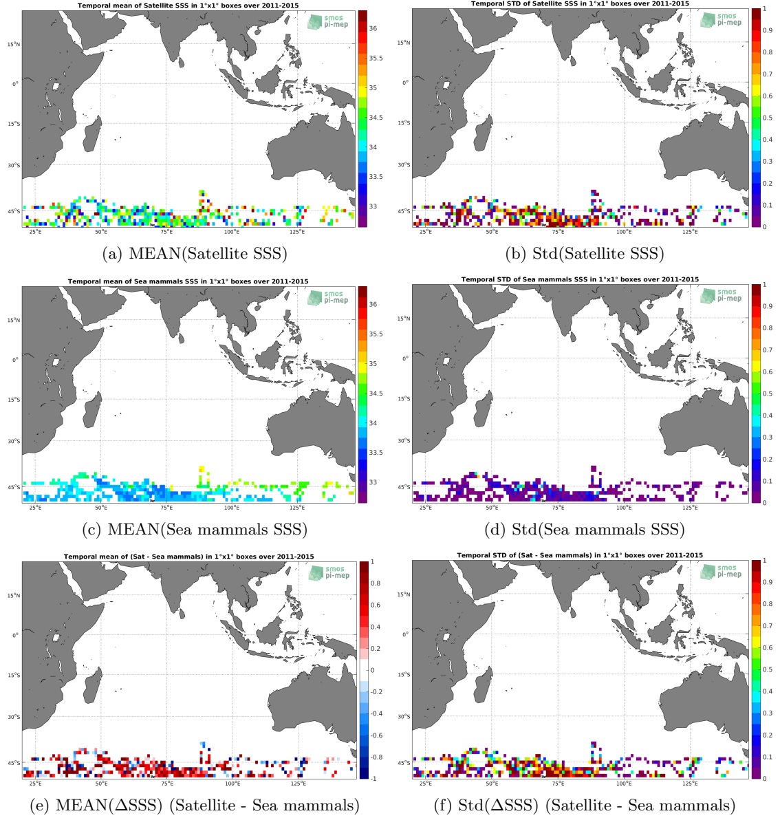
Figure 6: Temporal mean (left) and Std (right) of SSS from Aquarius-L2-JPL-V5 (top), Sea mammals (middle), and of \Delta SSS (Satellite - Sea mammals). Only match-up pairs are used to generate these maps.
