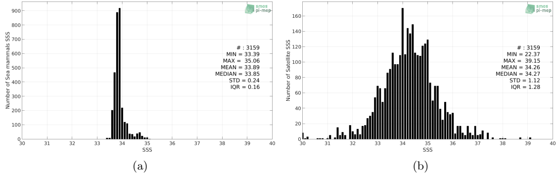
Figure 2: Histograms of SSS from Sea mammals (a) and Aquarius-L2-JPL-V5 (b) considering all match-up pairs per bins of 0.1 over the Indian Ocean Pi-MEP region and for the full satellite product period.
