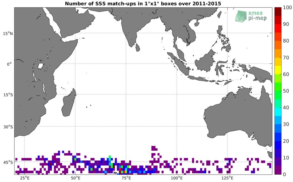
Figure 4: Number of SSS match-ups between Sea mammals SSS and the Aquarius-L2-JPL-V5 SSS product for the Indian Ocean Pi-MEP region over 1^\circ \times 1^\circ boxes and for the full satellite product period.
