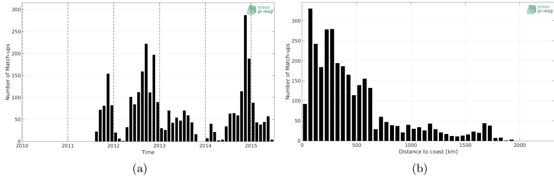
Figure 1: Number of match-ups between Sea mammals and Aquarius-L2-JPL-V5 SSS as a function of time (a) and as function of the distance to coast (b) over the Indian Ocean Pi-MEP region and for the full satellite product period.
