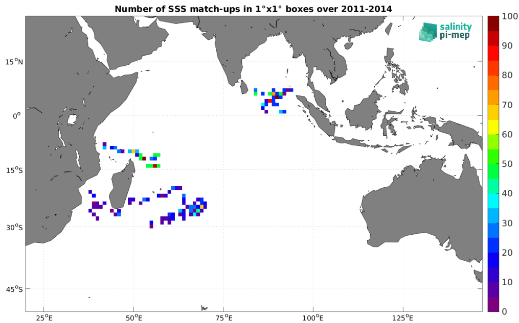
Figure 4: Number of SSS match-ups between Surface drifters SSS and the Aquarius SSS L2 CAP v5 (JPL) SSS product for the Indian Ocean Pi-MEP region over 1^\circ \times 1^\circ boxes and for the full satellite product period.
