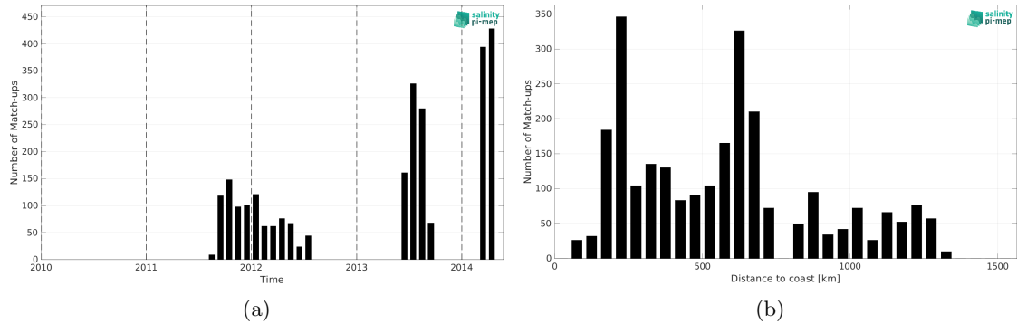
Figure 2: Number of match-ups between Surface drifters and Aquarius SSS L2 CAP v5 (JPL) SSS as a function of time (a) and as function of the distance to coast (b) over the Indian Ocean Pi-MEP region and for the full satellite product period.
