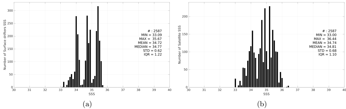
Figure 3: Histograms of SSS from Surface drifters (a) and Aquarius SSS L2 CAP v5 (JPL) (b) considering all match-up pairs per bins of 0.1 over the Indian Ocean Pi-MEP region and for the full satellite product period.
