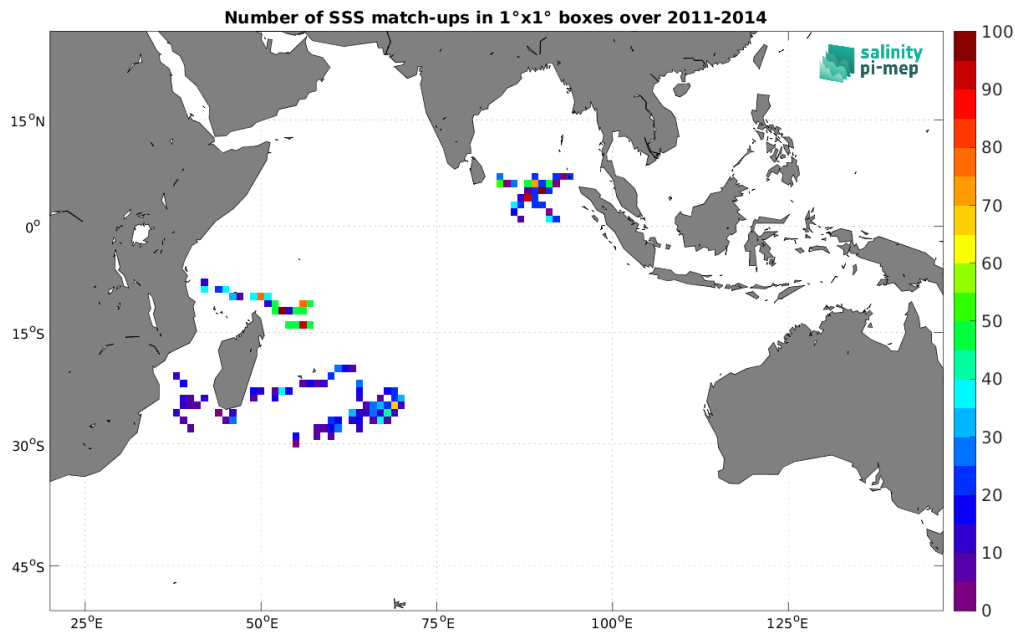
Figure 3: Number of SSS match-ups between Surface drifters SSS and the Aquarius SSS L2 CAP v5 (JPL) SSS product for the Indian Ocean Pi-MEP region over 1^\circ \times 1^\circ boxes and for the full satellite product period.
