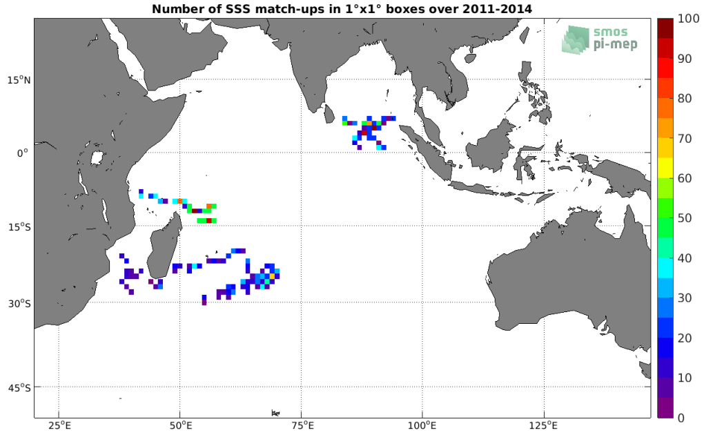
Figure 3: Number of SSS match-ups between Surface drifters SSS and the Aquarius SSS L2 CAP v5 (JPL) SSS product for the Indian Ocean Pi-MEP region over 1°x1° boxes and for the full satellite product period.
