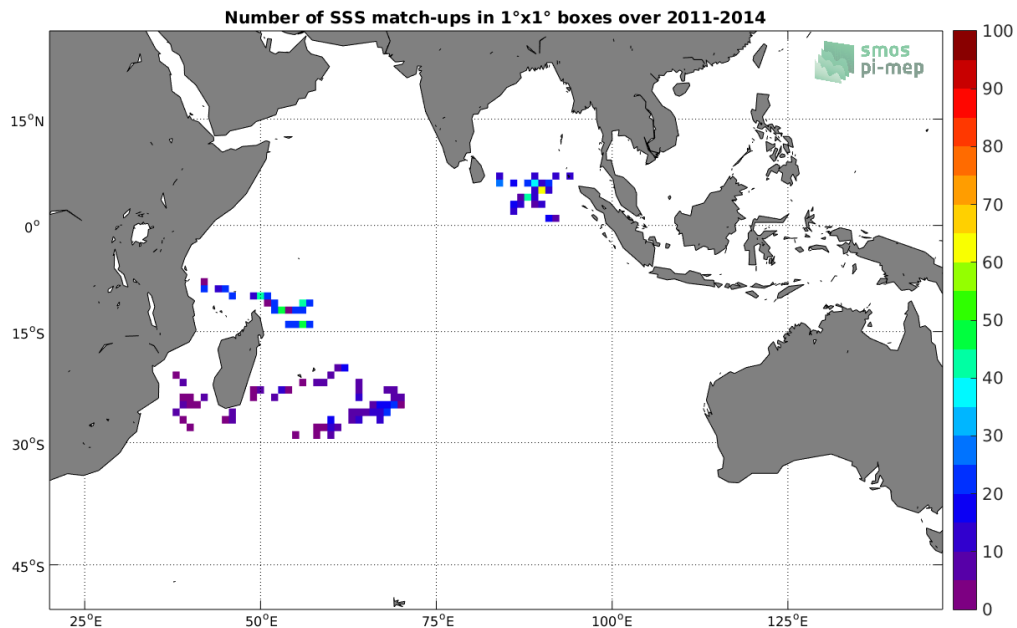
Figure 3: Number of SSS match-ups between Surface drifters SSS and the Aquarius-L2-JPL-V5 SSS product for the Indian Ocean Pi-MEP region over 1°x1° boxes and for the full satellite product period.
