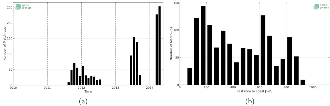
Figure 1: Number of match-ups between Surface drifters and Aquarius-L2-JPL-V5 SSS as a function of time (a) and as function of the distance to coast (b) over the Indian Ocean Pi-MEP region and for the full satellite product period.
