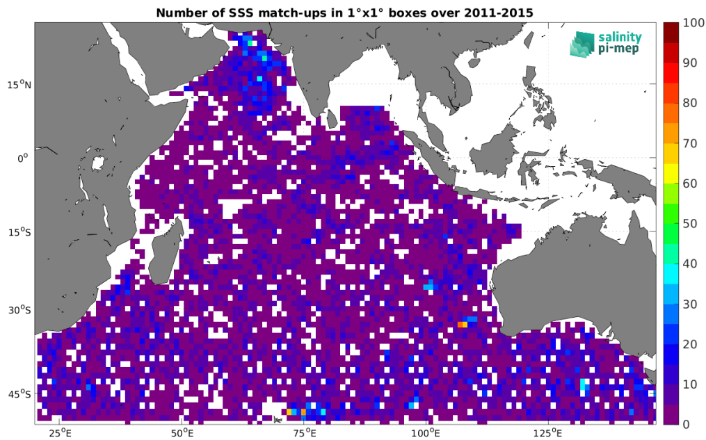
Figure 4: Number of SSS match-ups between Argo SSS and the Aquarius SSS L2 CAP v5 (JPL) SSS product for the Indian Ocean Pi-MEP region over 1^\circ \times 1^\circ boxes and for the full satellite product period.
