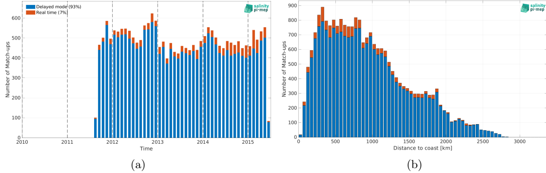
Figure 1: Number of match-ups between Argo and Aquarius SSS L2 CAP v5 (JPL) SSS as a function of time (a) and as function of the distance to coast (b) over the Indian Ocean Pi-MEP region and for the full satellite product period.
