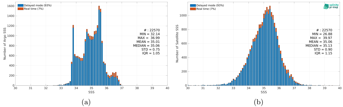
Figure 2: Histograms of SSS from Argo (a) and Aquarius SSS L2 CAP v5 (JPL) (b) considering all match-up pairs per bins of 0.1 over the Indian Ocean Pi-MEP region and for the full satellite product period.
