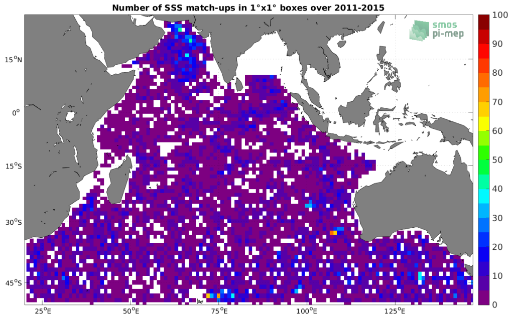
Figure 4: Number of SSS match-ups between Argo SSS and the Aquarius SSS L2 CAP v5 (JPL) SSS product for the Indian Ocean Pi-MEP region over 1^\circ \times 1^\circ boxes and for the full satellite product period.
