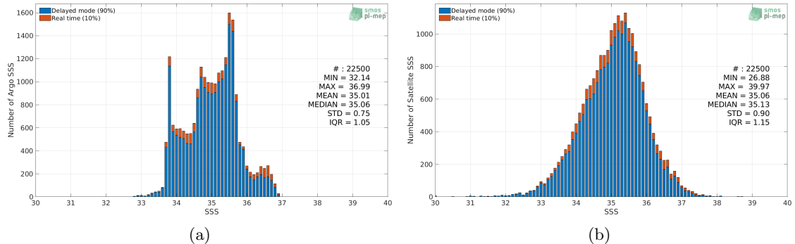
Figure 2: Histograms of SSS from Argo (a) and Aquarius SSS L2 CAP v5 (JPL) (b) considering all match-up pairs per bins of 0.1 over the Indian Ocean Pi-MEP region and for the full satellite product period.
