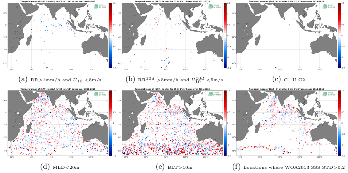
Figure 12: Temporal mean gridded over spatial boxes of size 1^\circ \times 1^\circ of \Delta\text{SSS} (Aquarius-L2-JPL-V5 - Argo) for 6 different subdatasets corresponding to: RR > 1\text{mm/h} and U_{10} < 5\text{m/s} (a), RR^{10d} > 5\text{mm/h} and U_{10}^{10d} < 5\text{m/s} (b), C1 U C2 (c), MLD < 20\text{m} (d), BLT > 10\text{m} (e), Locations where WOA2013 SSS STD > 0.2 (f).
