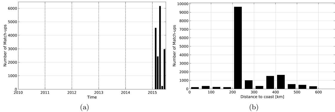
Figure 1: Number of match-ups between TSG-SAMOS and AQUARIUS-L2-JPL-V4 SSS as a function of time (a) and as function of the distance to coast (b) over the Indian Ocean Pi-MEP region and for the full satellite product period.
