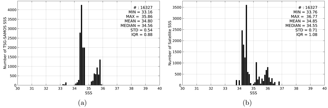
Figure 2: Histograms of SSS from TSG-SAMOS (a) and AQUARIUS-L2-JPL-V4 (b) considering all match-up pairs per bins of 0.1 over the Indian Ocean Pi-MEP region and for the full satellite product period.
