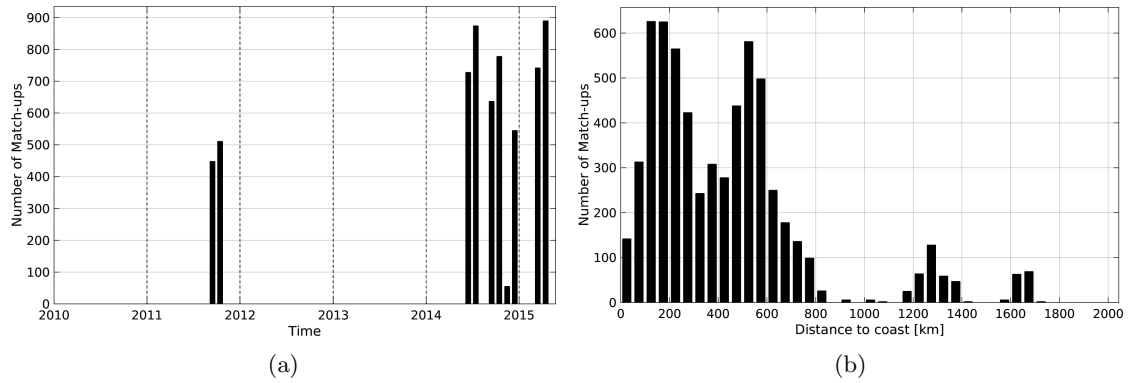
Figure 1: Number of match-ups between TSG-LEGOS-DM and AQUARIUS-L2-JPL-V4 SSS as a function of time (a) and as function of the distance to coast (b) over the Indian Ocean Pi-MEP region and for the full satellite product period.
