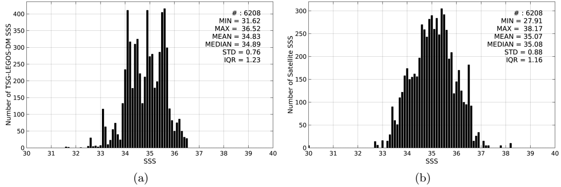
Figure 2: Histograms of SSS from TSG-LEGOS-DM (a) and AQUARIUS-L2-JPL-V4 (b) considering all match-up pairs per bins of 0.1 over the Indian Ocean Pi-MEP region and for the full satellite product period.
