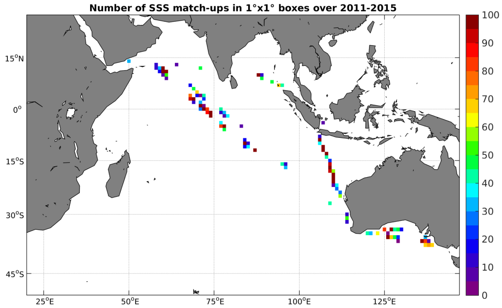
Figure 4: Number of SSS match-ups between TSG-LEGOS-DM SSS and the AQUARIUS-L2-JPL-V4 SSS product for the Indian Ocean Pi-MEP region over 1°x1° boxes and for the full satellite product period.
