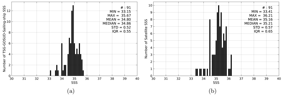
Figure 2: Histograms of SSS from TSG-GOSUD-Sailing-ship (a) and AQUARIUS-L2-JPL-V4 (b) considering all match-up pairs per bins of 0.1 over the Indian Ocean Pi-MEP region and for the full satellite product period.
