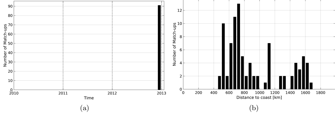
Figure 1: Number of match-ups between TSG-GOSUD-Sailing-ship and AQUARIUS-L2-JPL-V4 SSS as a function of time (a) and as function of the distance to coast (b) over the Indian Ocean Pi-MEP region and for the full satellite product period.
