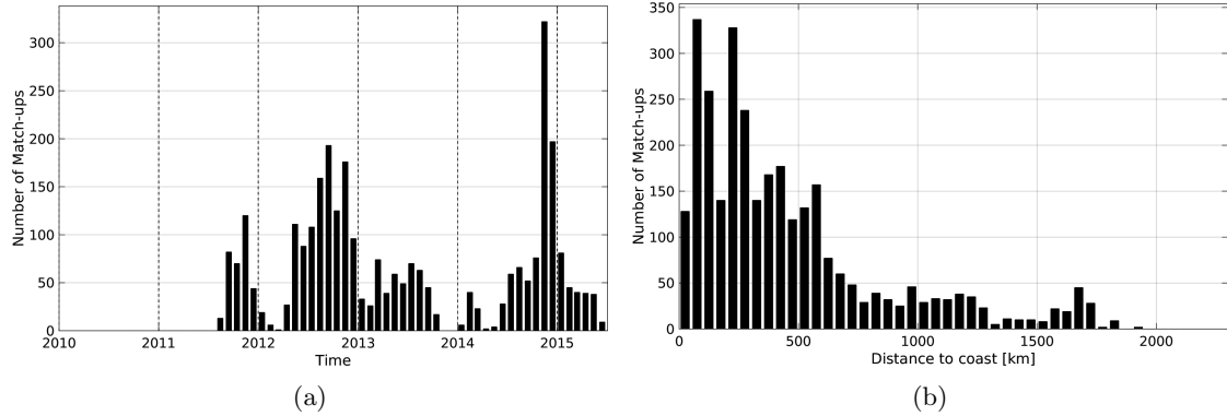
Figure 1: Number of match-ups between Sea mammals and AQUARIUS-L2-JPL-V4 SSS as a function of time (a) and as function of the distance to coast (b) over the Indian Ocean Pi-MEP region and for the full satellite product period.
