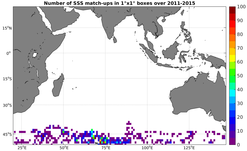
Figure 4: Number of SSS match-ups between Sea mammals SSS and the AQUARIUS-L2-JPL-V4 SSS product for the Indian Ocean Pi-MEP region over 1^\circ \times 1^\circ boxes and for the full satellite product period.
