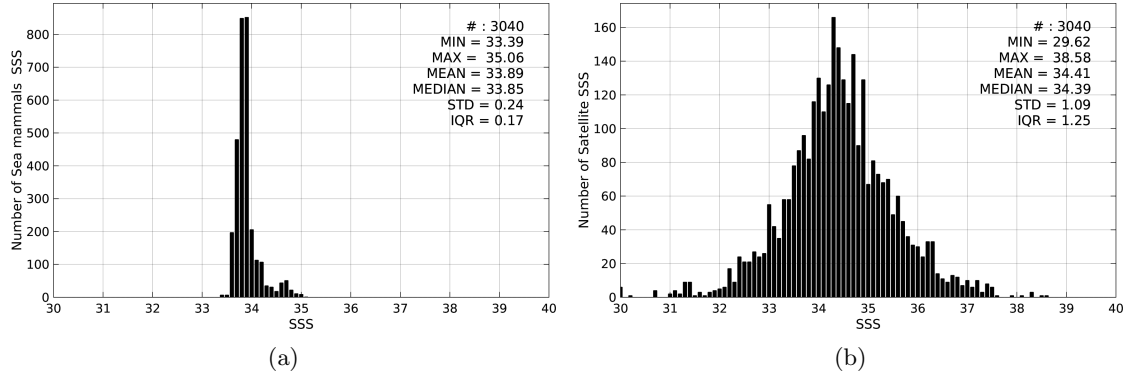
Figure 2: Histograms of SSS from Sea mammals (a) and AQUARIUS-L2-JPL-V4 (b) considering all match-up pairs per bins of 0.1 over the Indian Ocean Pi-MEP region and for the full satellite product period.
