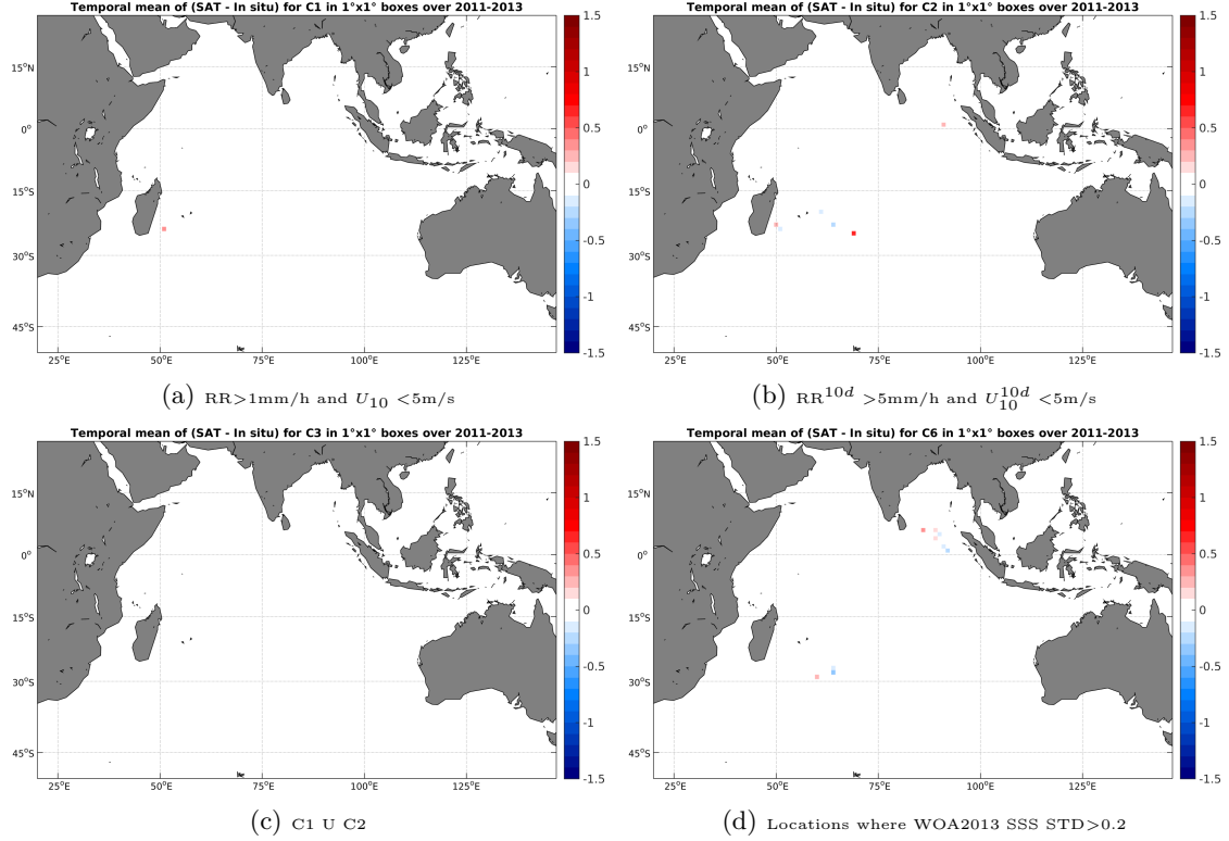
Figure 11: Temporal mean gridded over spatial boxes of size 1^\circ \times 1^\circ of \Delta SSS (AQUARIUS-L2-JPL-V4 - Surface drifters) for 4 different subdatasets corresponding to: RR > 1 mm/h and U_{10} < 5 m/s (a), RR^{10d} > 5 mm/h and U_{10}^{10d} < 5 m/s (b), C1 U C2 (c), Locations where WOA2013 SSS STD > 0.2 (d).
