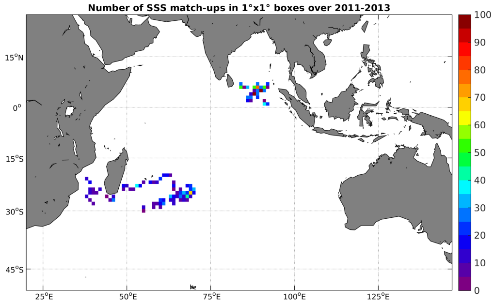
Figure 3: Number of SSS match-ups between Surface drifters SSS and the AQUARIUS-L2-JPL-V4 SSS product for the Indian Ocean Pi-MEP region over 1°x1° boxes and for the full satellite product period.
