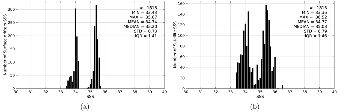
Figure 2: Histograms of SSS from Surface drifters (a) and AQUARIUS-L2-JPL-V4 (b) considering all match-up pairs per bins of 0.1 over the Indian Ocean Pi-MEP region and for the full satellite product period.
