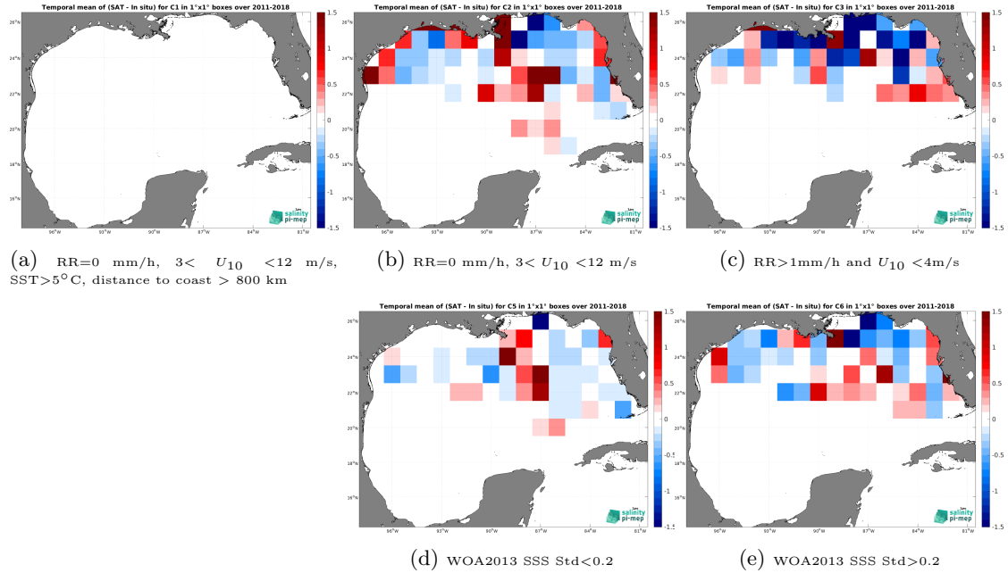
Figure 12: Temporal mean gridded over spatial boxes of size 1^{\circ}\times 1^{\circ} of \Delta\text{SSS} (SMOS and SMAP SSS L4 OI v1 - 7 Days (LOPS) - TSG (SAMOS)) for 5 different subdatasets corresponding to:RR=0 mm/h, 3 < U_{10} < 12 m/s, SST >5^{\circ}\text{C} , distance to coast > 800 km (a), RR=0 mm/h, 3 < U_{10} < 12 m/s (b), RR >1 mm/h and U_{10} < 4 m/s (c), WOA2013 SSS Std <0.2 (d), WOA2013 SSS Std >0.2 (e).
