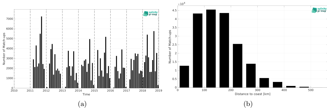
Figure 1: Number of match-ups between TSG (SAMOS) and SMOS and SMAP SSS L4 OI v1 - 7 Days (LOPS) SSS as a function of time (a) and as function of the distance to coast (b) over the Gulf of Mexico Pi-MEP region and for the full satellite product period.
