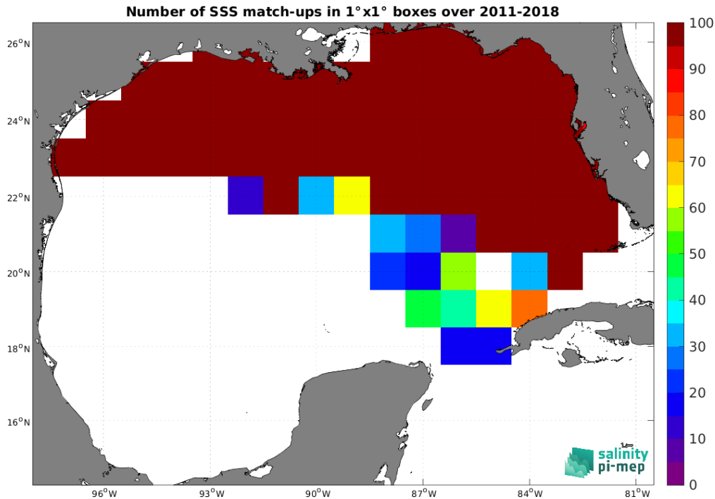
Figure 4: Number of SSS match-ups between TSG (SAMOS) SSS and the SMOS and SMAP SSS L4 OI v1 - 7 Days (LOPS) SSS product for the Gulf of Mexico Pi-MEP region over 1^\circ \times 1^\circ boxes and for the full satellite product period.
