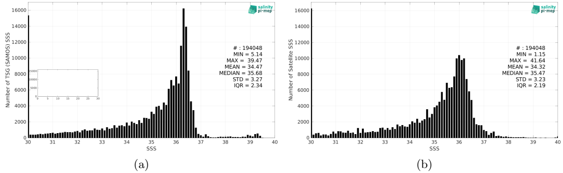
Figure 2: Histograms of SSS from TSG (SAMOS) (a) and SMOS and SMAP SSS L4 OI v1 - 7 Days (LOPS) (b) considering all match-up pairs per bins of 0.1 over the Gulf of Mexico Pi-MEP region and for the full satellite product period.
