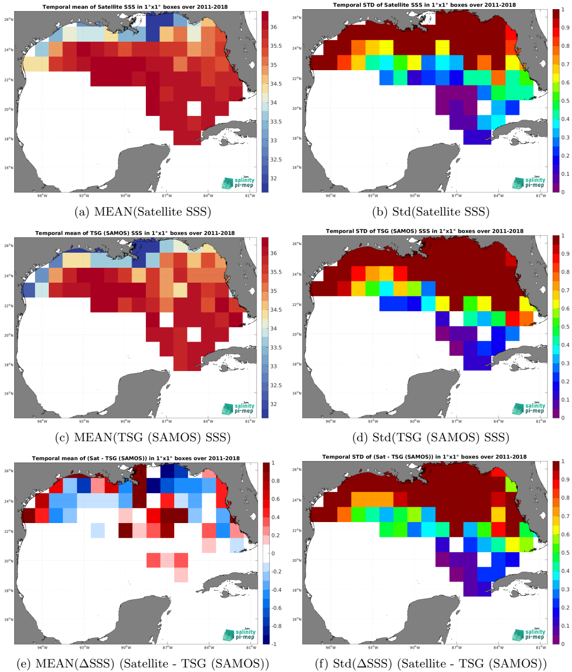
Figure 6: Temporal mean (left) and Std (right) of SSS from SMOS and SMAP SSS L4 OI v1 - 7 Days (LOPS) (top), TSG (SAMOS) (middle), and of \Delta SSS (Satellite - TSG (SAMOS)). Only match-up pairs are used to generate these maps.
