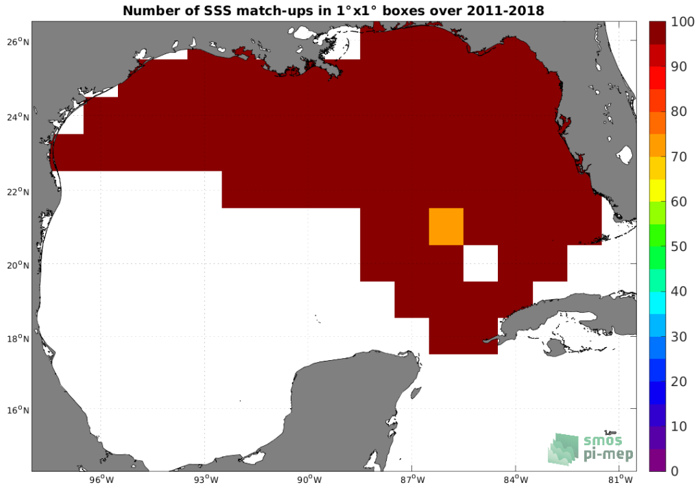
Figure 4: Number of SSS match-ups between TSG (SAMOS) SSS and the SMOS and SMAP SSS L4 OI v1 - 7 Days (LOPS) SSS product for the Gulf of Mexico Pi-MEP region over 1^{\circ} \times 1^{\circ} boxes and for the full satellite product period.
