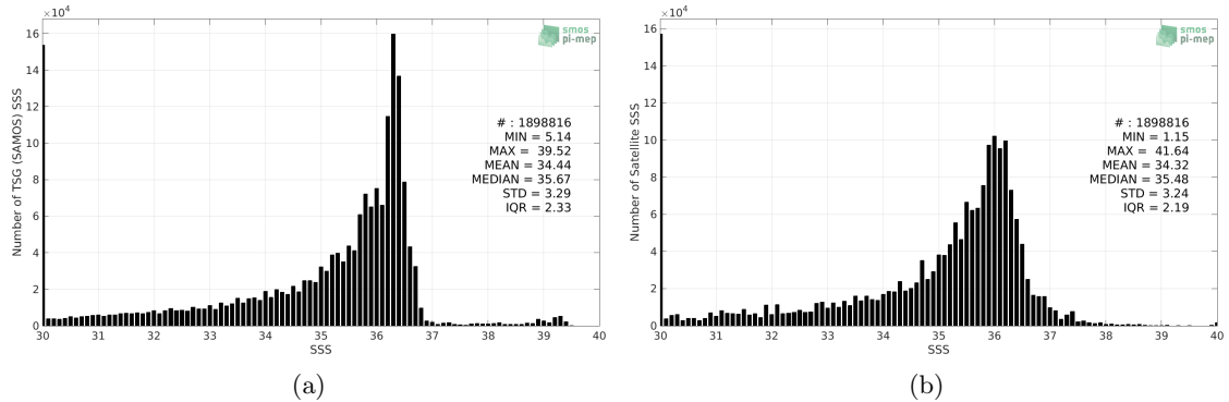
Figure 2: Histograms of SSS from TSG (SAMOS) (a) and SMOS and SMAP SSS L4 OI v1 - 7 Days (LOPS) (b) considering all match-up pairs per bins of 0.1 over the Gulf of Mexico Pi-MEP region and for the full satellite product period.
