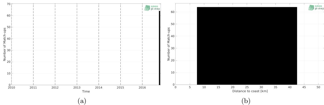
Figure 1: Number of match-ups between TSG (LEGOS-DM) and SMOS and SMAP SSS L4 OI v1 - 7 Days (LOPS) SSS as a function of time (a) and as function of the distance to coast (b) over the Gulf of Mexico Pi-MEP region and for the full satellite product period.
