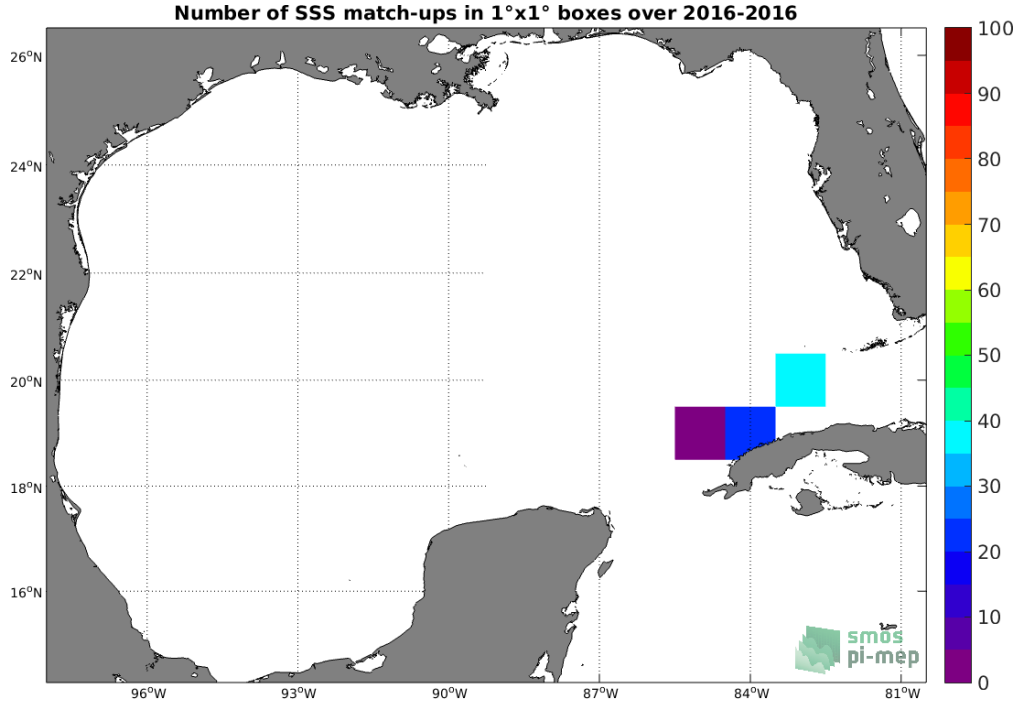
Figure 4: Number of SSS match-ups between TSG (LEGOS-DM) SSS and the SMOS and SMAP SSS L4 OI v1 - 7 Days (LOPS) SSS product for the Gulf of Mexico Pi-MEP region over 1^\circ \times 1^\circ boxes and for the full satellite product period.
