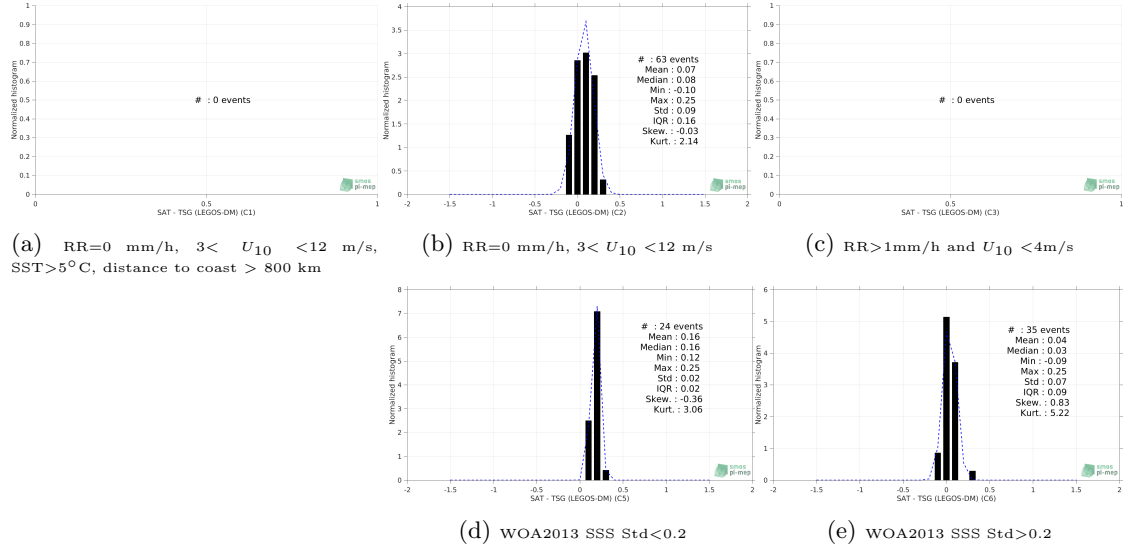
Figure 13: Normalized histogram of \Delta\text{SSS} (SMOS and SMAP SSS L4 OI v1 - 7 Days (LOPS) - TSG (LEGOS-DM)) for 5 different subdatasets corresponding to: RR=0 mm/h, 3 < U_{10} < 12 m/s, SST > 5^\circ\text{C} , distance to coast > 800 km (a), RR=0 mm/h, 3 < U_{10} < 12 m/s (b), RR > 1\text{mm/h} and U_{10} < 4\text{m/s} (c), WOA2013 SSS Std < 0.2 (d), WOA2013 SSS Std > 0.2 (e).
