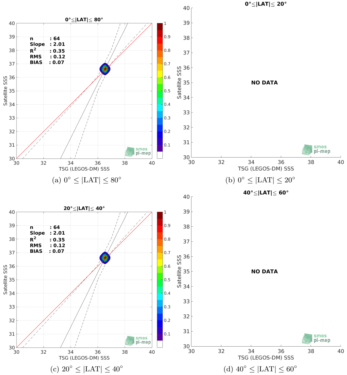
Figure 9: Contour maps of the concentration of SMOS and SMAP SSS L4 OI v1 - 7 Days (LOPS) SSS (y-axis) versus TSG (LEGOS-DM) SSS (x-axis) at match-up pairs for different latitude bands. For each plot, the red line shows x=y . The black thin and dashed lines indicate a linear fit through the data cloud and the \pm 95\% confidence levels, respectively. The number match-up pairs n , the slope and R^2 coefficient of the linear fit, the root mean square (RMS) and the mean bias between satellite and in situ data are indicated for each latitude band in each plots.
