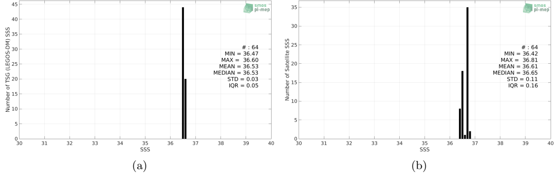
Figure 2: Histograms of SSS from TSG (LEGOS-DM) (a) and SMOS and SMAP SSS L4 OI v1 - 7 Days (LOPS) (b) considering all match-up pairs per bins of 0.1 over the Gulf of Mexico Pi-MEP region and for the full satellite product period.
