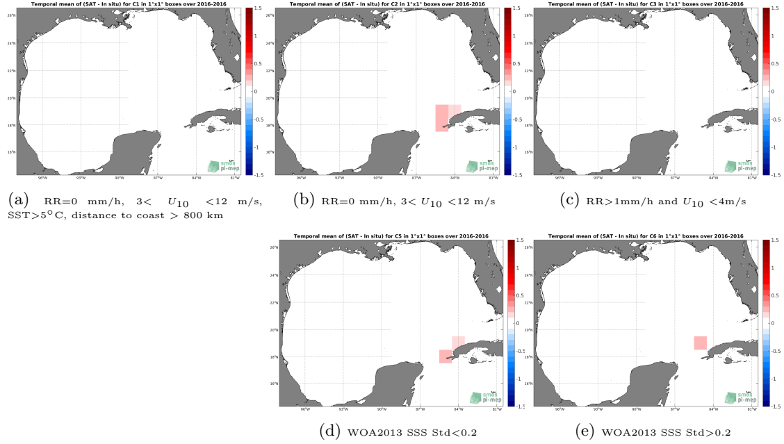
Figure 12: Temporal mean gridded over spatial boxes of size 1^{\circ}\times 1^{\circ} of \Delta\text{SSS} (SMOS and SMAP SSS L4 OI v1 - 7 Days (LOPS) - TSG (LEGOS-DM)) for 5 different subdatasets corresponding to:RR=0 mm/h, 3 < U_{10} < 12 m/s, SST >5^{\circ}\text{C} , distance to coast > 800 km (a), RR=0 mm/h, 3 < U_{10} < 12 m/s (b), RR >1 mm/h and U_{10} < 4 m/s (c), WOA2013 SSS Std <0.2 (d), WOA2013 SSS Std >0.2 (e).
