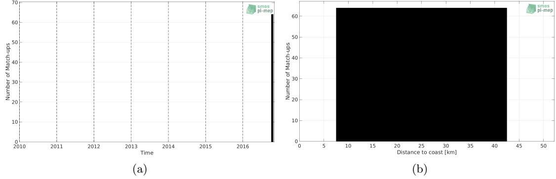
Figure 1: Number of match-ups between TSG (LEGOS-DM) and SMOS and SMAP SSS L4 OI v1 - 7 Days (LOPS) SSS as a function of time (a) and as function of the distance to coast (b) over the Gulf of Mexico Pi-MEP region and for the full satellite product period.
