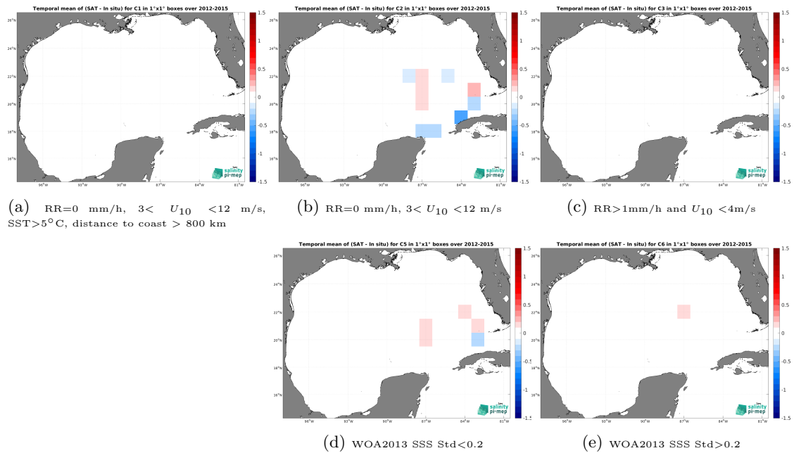
Figure 12: Temporal mean gridded over spatial boxes of size 1^{\circ}\times 1^{\circ} of \Delta SSS (SMOS and SMAP SSS L4 OI v1 - 7 Days (LOPS) - TSG (GOSUD-Sailing-ship)) for 5 different subdatasets corresponding to:RR=0 mm/h, 3 < U_{10} < 12 m/s, SST >5^{\circ}\text{C} , distance to coast > 800 km (a), RR=0 mm/h, 3 < U_{10} < 12 m/s (b), RR >1 mm/h and U_{10} < 4 m/s (c), WOA2013 SSS Std <0.2 (d), WOA2013 SSS Std >0.2 (e).
