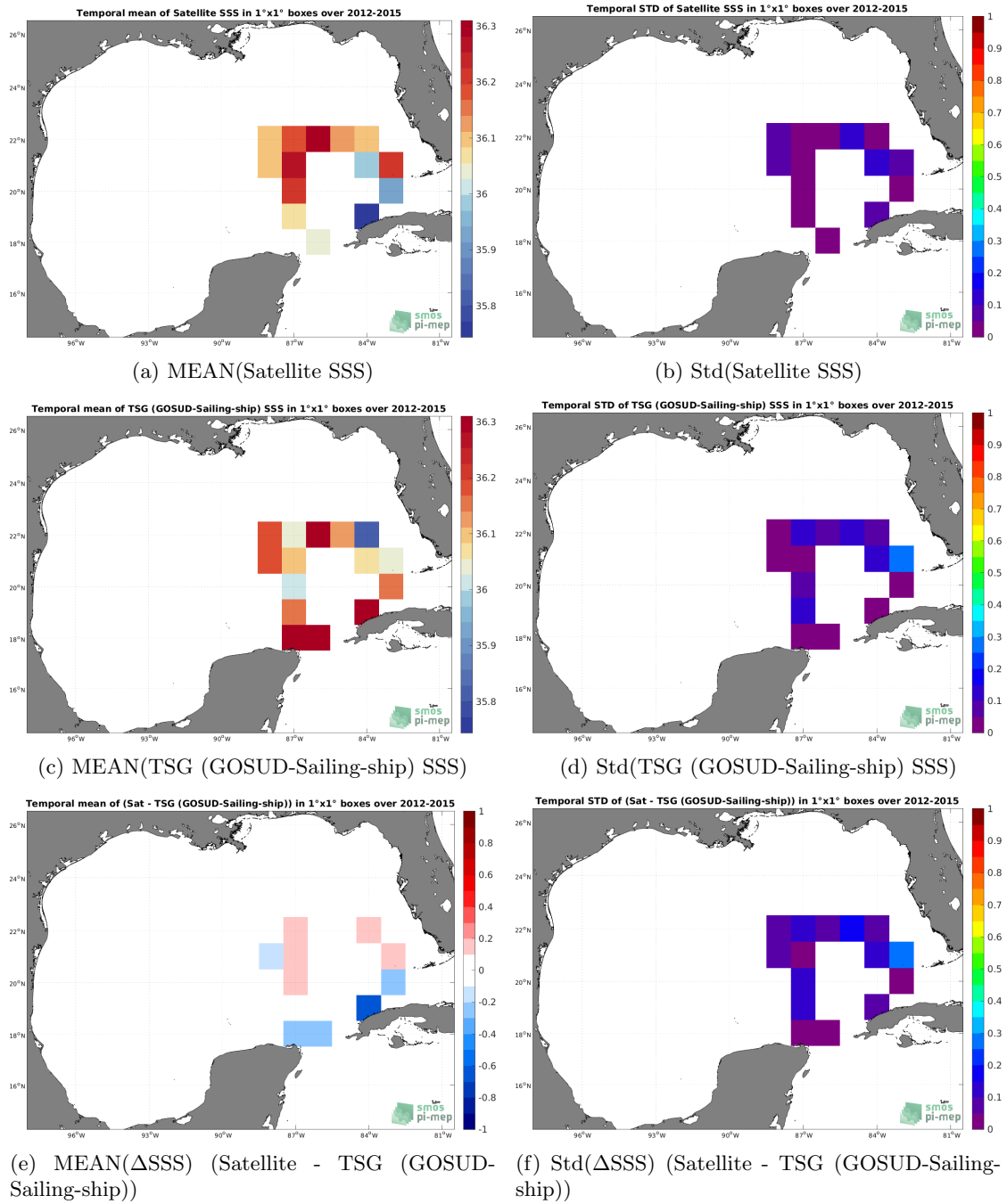
Figure 6: Temporal mean (left) and Std (right) of SSS from SMOS and SMAP SSS L4 OI v1 - 7 Days (LOPS) (top), TSG (GOSUD-Sailing-ship) (middle), and of \Delta SSS (Satellite - TSG (GOSUD-Sailing-ship)). Only match-up pairs are used to generate these maps.
