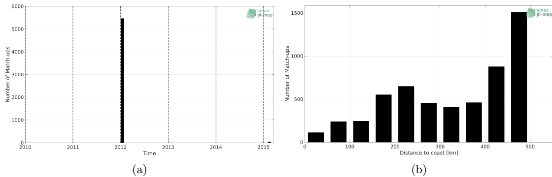
Figure 1: Number of match-ups between TSG (GOSUD-Sailing-ship) and SMOS and SMAP SSS L4 OI v1 - 7 Days (LOPS) SSS as a function of time (a) and as function of the distance to coast (b) over the Gulf of Mexico Pi-MEP region and for the full satellite product period.
