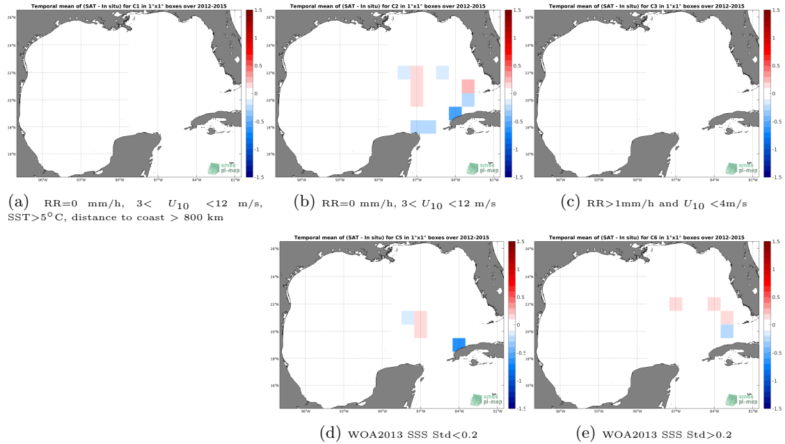
Figure 12: Temporal mean gridded over spatial boxes of size 1^\circ \times 1^\circ of \Delta SSS (SMOS and SMAP SSS L4 OI v1 - 7 Days (LOPS) - TSG (GOSUD-Sailing-ship)) for 5 different subdatasets corresponding to:RR=0 mm/h, 3 < U_{10} < 12 m/s, SST >5^\circ\text{C} , distance to coast > 800 km (a), RR=0 mm/h, 3 < U_{10} < 12 m/s (b), RR >1 mm/h and U_{10} < 4 m/s (c), WOA2013 SSS Std <0.2 (d), WOA2013 SSS Std >0.2 (e).
