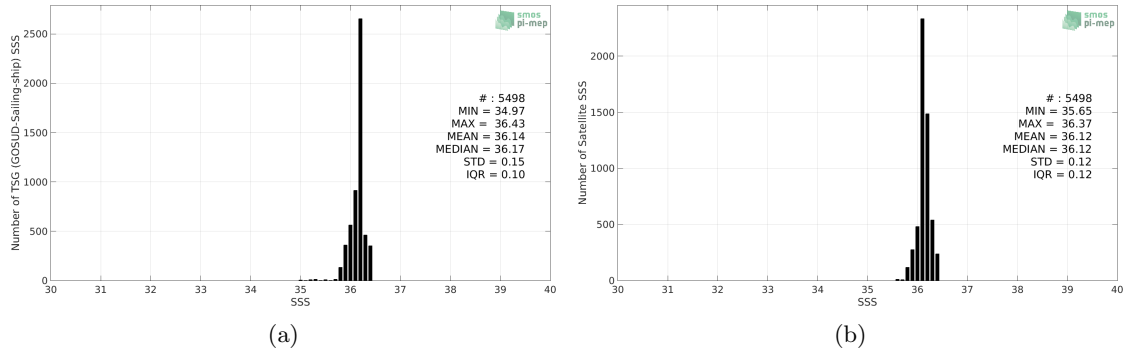
Figure 2: Histograms of SSS from TSG (GOSUD-Sailing-ship) (a) and SMOS and SMAP SSS L4 OI v1 - 7 Days (LOPS) (b) considering all match-up pairs per bins of 0.1 over the Gulf of Mexico Pi-MEP region and for the full satellite product period.
