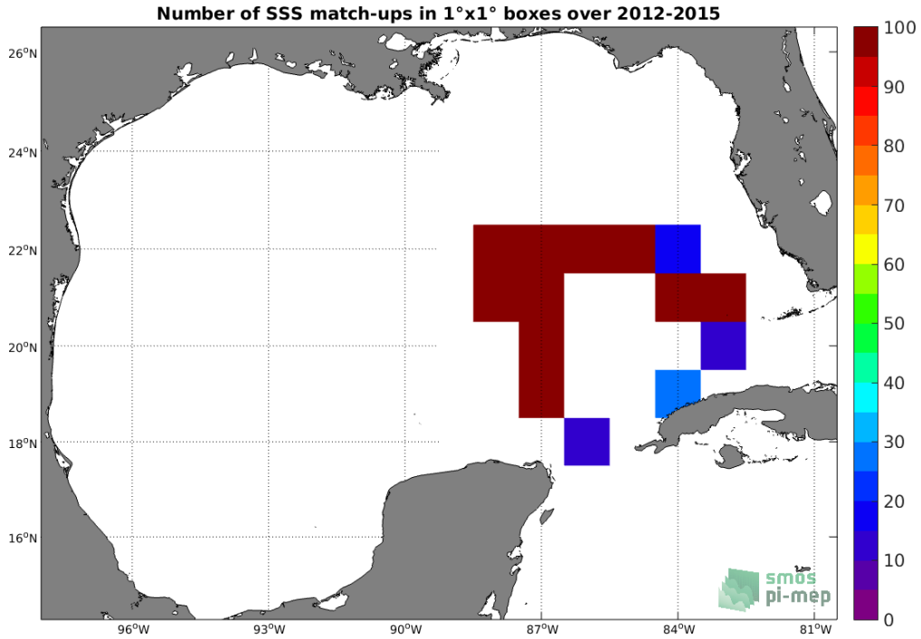
Figure 4: Number of SSS match-ups between TSG (GOSUD-Sailing-ship) SSS and the SMOS and SMAP SSS L4 OI v1 - 7 Days (LOPS) SSS product for the Gulf of Mexico Pi-MEP region over 1^\circ \times 1^\circ boxes and for the full satellite product period.
