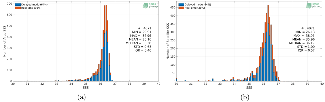
Figure 2: Histograms of SSS from Argo (a) and SMOS and SMAP SSS L4 OI v1 - 7 Days (LOPS) (b) considering all match-up pairs per bins of 0.1 over the Gulf of Mexico Pi-MEP region and for the full satellite product period.
