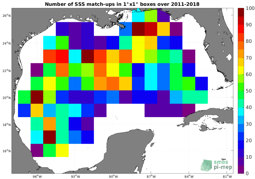
Figure 4: Number of SSS match-ups between Argo SSS and the SMOS and SMAP SSS L4 OI v1 - 7 Days (LOPS) SSS product for the Gulf of Mexico Pi-MEP region over 1^\circ \times 1^\circ boxes and for the full satellite product period.
