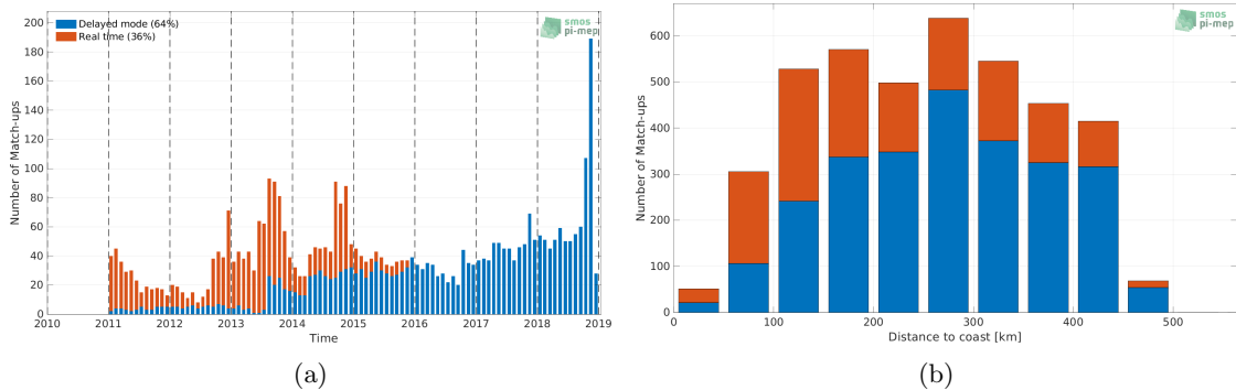
Figure 1: Number of match-ups between Argo and SMOS and SMAP SSS L4 OI v1 - 7 Days (LOPS) SSS as a function of time (a) and as function of the distance to coast (b) over the Gulf of Mexico Pi-MEP region and for the full satellite product period.
