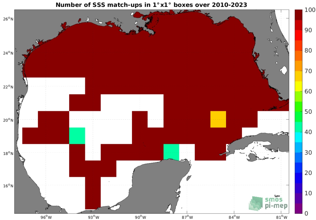
Figure 4: Number of SSS match-ups between TSG (SAMOS) SSS and the SMOS SSS L4 v1 - Weekly (CMEMS-CNR) SSS product for the Gulf of Mexico Pi-MEP region over 1^\circ \times 1^\circ boxes and for the full satellite product period.
