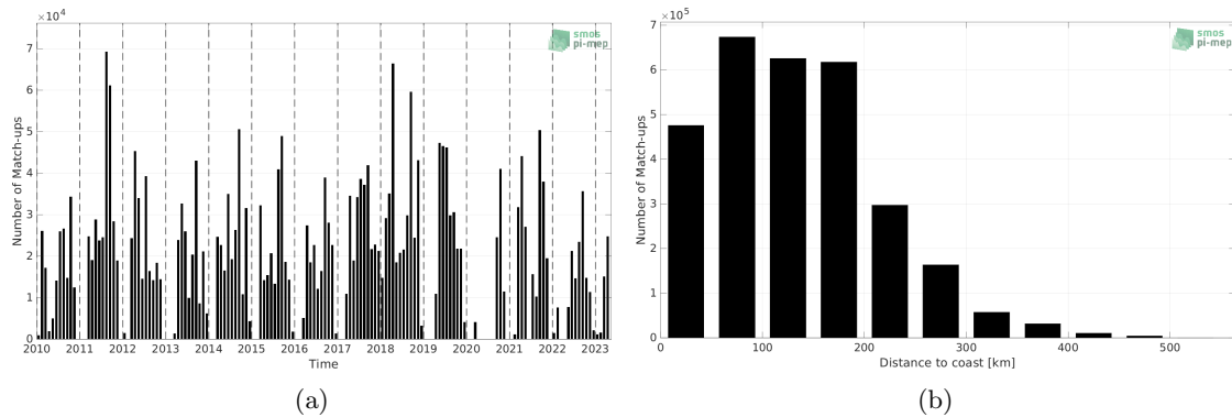
Figure 1: Number of match-ups between TSG (SAMOS) and SMOS SSS L4 v1 - Weekly (CMEMS-CNR) SSS as a function of time (a) and as function of the distance to coast (b) over the Gulf of Mexico Pi-MEP region and for the full satellite product period.
