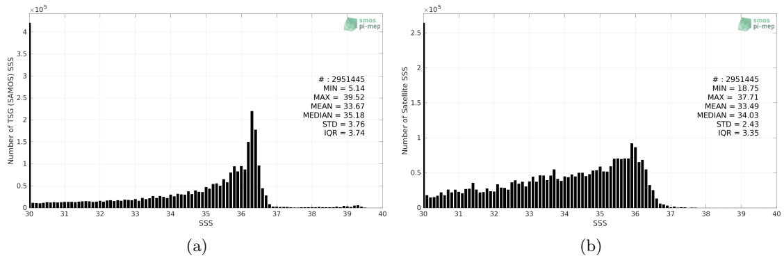
Figure 2: Histograms of SSS from TSG (SAMOS) (a) and SMOS SSS L4 v1 - Weekly (CMEMS-CNR) (b) considering all match-up pairs per bins of 0.1 over the Gulf of Mexico Pi-MEP region and for the full satellite product period.
