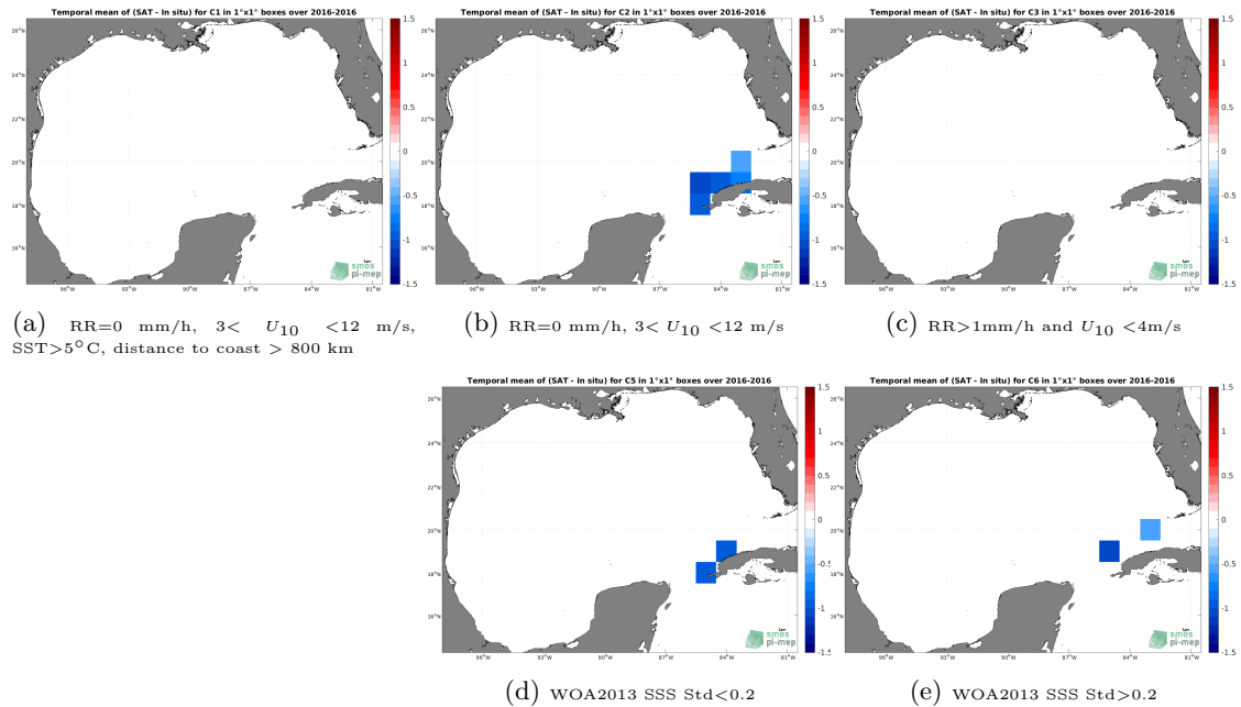
Figure 12: Temporal mean gridded over spatial boxes of size 1^{\circ}\times 1^{\circ} of \Delta\text{SSS} (SMOS SSS L4 v1 - Weekly (CMEMS-CNR) - TSG (LEGOS-DM)) for 5 different subdatasets corresponding to:RR=0 mm/h, 3 < U_{10} < 12 m/s, SST >5^{\circ}\text{C} , distance to coast > 800 km (a), RR=0 mm/h, 3 < U_{10} < 12 m/s (b), RR >1 mm/h and U_{10} < 4 m/s (c), WOA2013 SSS Std <0.2 (d), WOA2013 SSS Std >0.2 (e).
