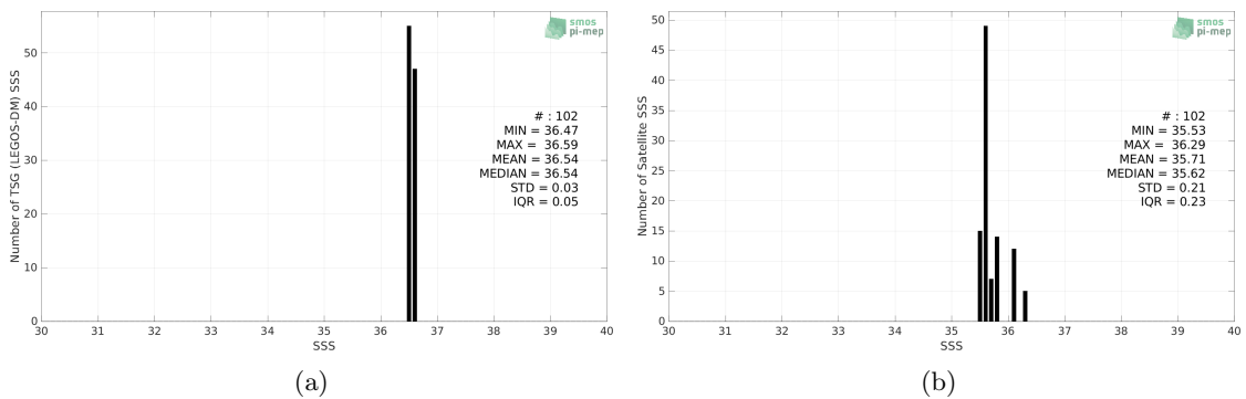
Figure 2: Histograms of SSS from TSG (LEGOS-DM) (a) and SMOS SSS L4 v1 - Weekly (CMEMS-CNR) (b) considering all match-up pairs per bins of 0.1 over the Gulf of Mexico Pi-MEP region and for the full satellite product period.
