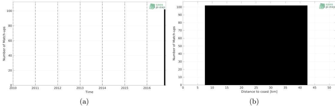
Figure 1: Number of match-ups between TSG (LEGOS-DM) and SMOS SSS L4 v1 - Weekly (CMEMS-CNR) SSS as a function of time (a) and as function of the distance to coast (b) over the Gulf of Mexico Pi-MEP region and for the full satellite product period.
