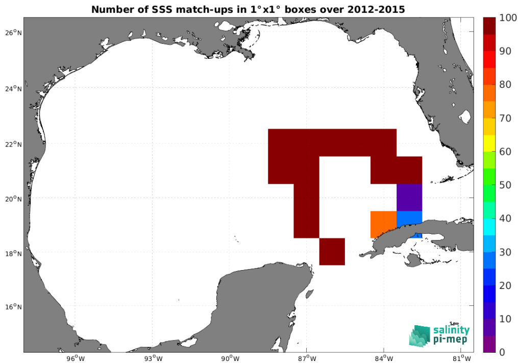
Figure 4: Number of SSS match-ups between TSG (GOSUD-Sailing-ship) SSS and the SMOS SSS L4 v1 - Weekly (CMEMS-CNR) SSS product for the Gulf of Mexico Pi-MEP region over 1^\circ \times 1^\circ boxes and for the full satellite product period.
