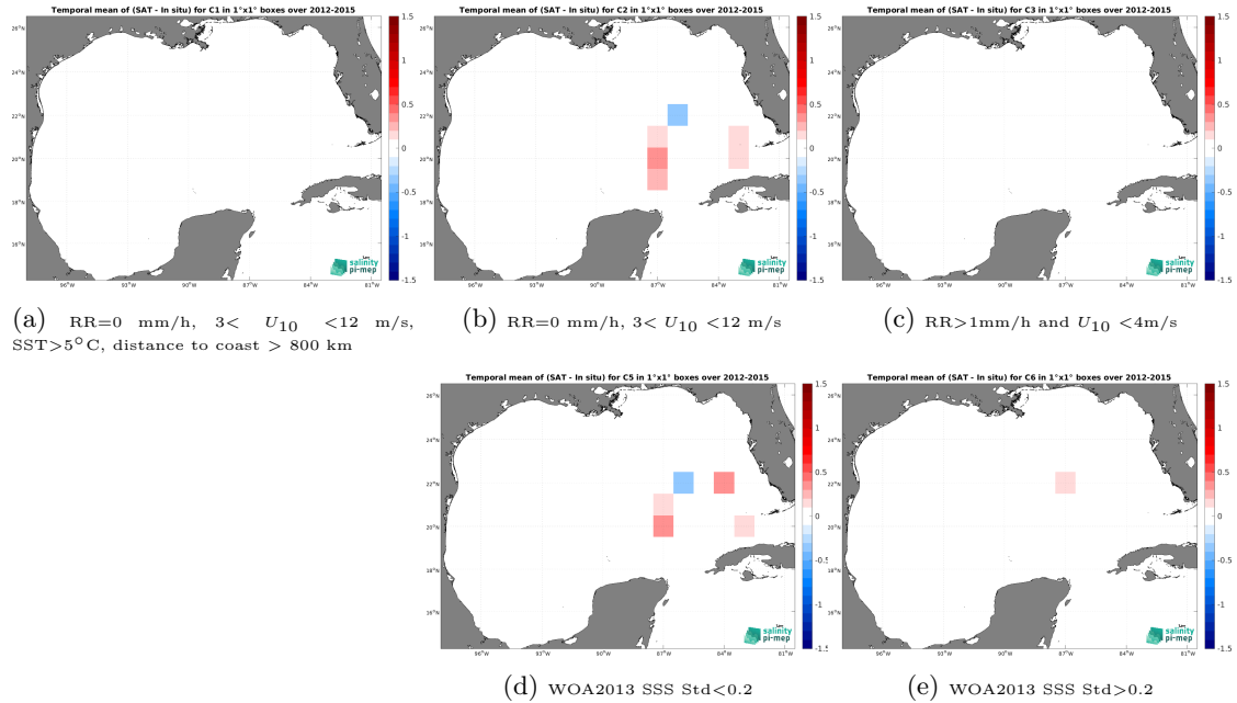
Figure 12: Temporal mean gridded over spatial boxes of size 1^{\circ}\times 1^{\circ} of \Delta SSS (SMOS SSS L4 v1 - Weekly (CMEMS-CNR) - TSG (GOSUD-Sailing-ship)) for 5 different subdatasets corresponding to:RR=0 mm/h, 3 < U_{10} < 12 m/s, SST >5^{\circ}\text{C} , distance to coast > 800 km (a), RR=0 mm/h, 3 < U_{10} < 12 m/s (b), RR >1 mm/h and U_{10} < 4 m/s (c), WOA2013 SSS Std <0.2 (d), WOA2013 SSS Std >0.2 (e).
