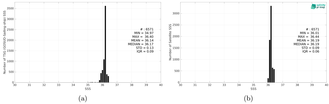
Figure 2: Histograms of SSS from TSG (GOSUD-Sailing-ship) (a) and SMOS SSS L4 v1 - Weekly (CMEMS-CNR) (b) considering all match-up pairs per bins of 0.1 over the Gulf of Mexico Pi-MEP region and for the full satellite product period.
