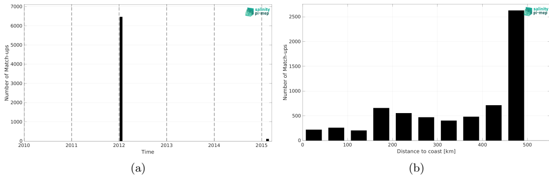
Figure 1: Number of match-ups between TSG (GOSUD-Sailing-ship) and SMOS SSS L4 v1 - Weekly (CMEMS-CNR) SSS as a function of time (a) and as function of the distance to coast (b) over the Gulf of Mexico Pi-MEP region and for the full satellite product period.
