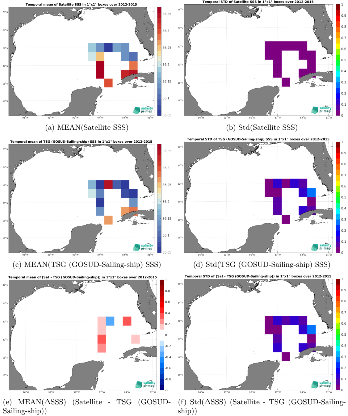
Figure 6: Temporal mean (left) and Std (right) of SSS from SMOS SSS L4 v1 - Weekly (CMEMS-CNR) (top), TSG (GOSUD-Sailing-ship) (middle), and of \Delta SSS (Satellite - TSG (GOSUD-Sailing-ship)). Only match-up pairs are used to generate these maps.
