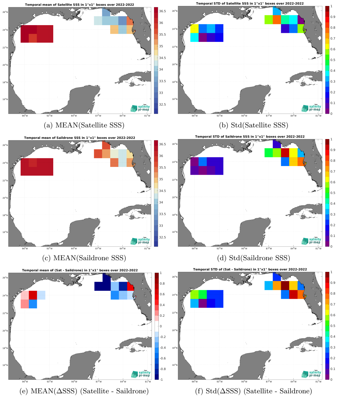
Figure 6: Temporal mean (left) and Std (right) of SSS from SMOS SSS L4 v1 - Weekly (CMEMS-CNR) (top), Saildrone (middle), and of \Delta SSS (Satellite - Saildrone). Only match-up pairs are used to generate these maps.
