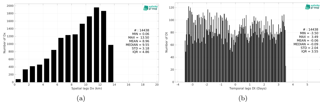
Figure 5: Histograms of the spatial (a) and temporal (b) lags between the location/time of the Saildrone measurements and the date of the corresponding SMOS SSS L4 v1 - Weekly (CMEMS-CNR) SSS pixel.
