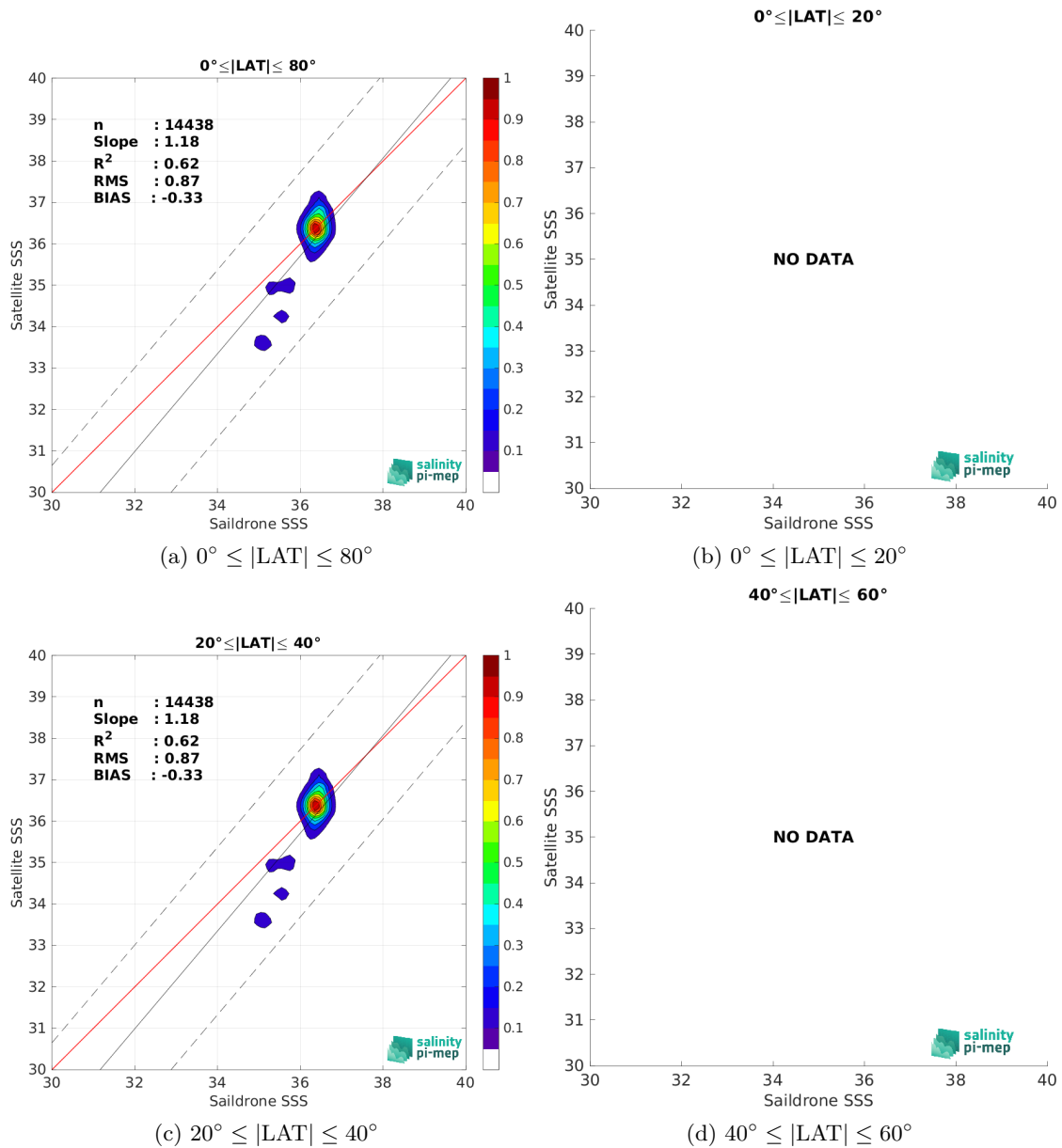
Figure 9: Contour maps of the concentration of SMOS SSS L4 v1 - Weekly (CMEMS-CNR) SSS (y-axis) versus Saildrone SSS (x-axis) at match-up pairs for different latitude bands. For each plot, the red line shows x=y . The black thin and dashed lines indicate a linear fit through the data cloud and the \pm 95\% confidence levels, respectively. The number match-up pairs n , the slope and R^2 coefficient of the linear fit, the root mean square (RMS) and the mean bias between satellite and in situ data are indicated for each latitude band in each plots.
