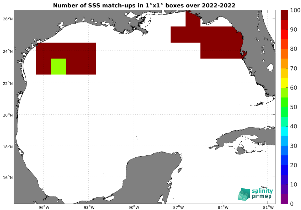
Figure 4: Number of SSS match-ups between Saildrone SSS and the SMOS SSS L4 v1 - Weekly (CMEMS-CNR) SSS product for the Gulf of Mexico Pi-MEP region over 1^\circ \times 1^\circ boxes and for the full satellite product period.
