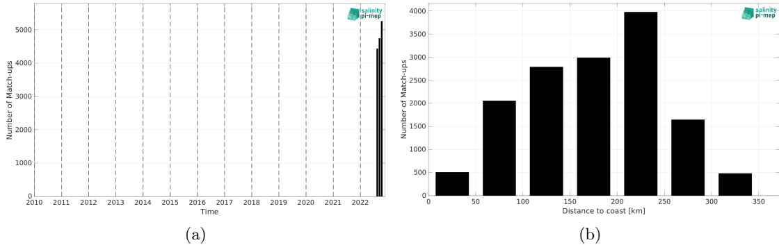
Figure 1: Number of match-ups between Saildrone and SMOS SSS L4 v1 - Weekly (CMEMS-CNR) SSS as a function of time (a) and as function of the distance to coast (b) over the Gulf of Mexico Pi-MEP region and for the full satellite product period.
