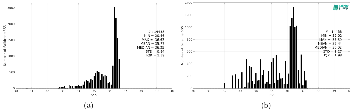
Figure 2: Histograms of SSS from Saildrone (a) and SMOS SSS L4 v1 - Weekly (CMEMS-CNR) (b) considering all match-up pairs per bins of 0.1 over the Gulf of Mexico Pi-MEP region and for the full satellite product period.
