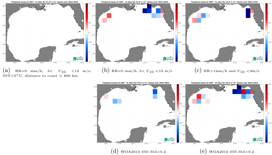
Figure 12: Temporal mean gridded over spatial boxes of size 1^{\circ}\times 1^{\circ} of \Delta\text{SSS} (SMOS SSS L4 v1 - Weekly (CMEMS-CNR) - Saildrone) for 5 different subdatasets corresponding to:RR=0 mm/h, 3 < U_{10} < 12 m/s, SST >5^{\circ}\text{C} , distance to coast > 800 km (a), RR=0 mm/h, 3 < U_{10} < 12 m/s (b), RR >1 mm/h and U_{10} < 4 m/s (c), WOA2013 SSS Std <0.2 (d), WOA2013 SSS Std >0.2 (e).
