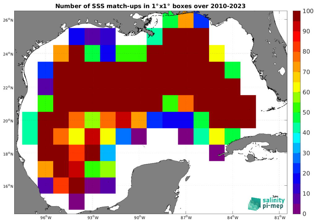
Figure 4: Number of SSS match-ups between Argo SSS and the SMOS SSS L4 v1 - Weekly (CMEMS-CNR) SSS product for the Gulf of Mexico Pi-MEP region over 1^\circ \times 1^\circ boxes and for the full satellite product period.
