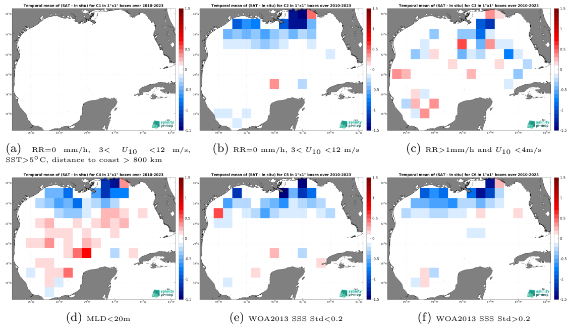
Figure 12: Temporal mean gridded over spatial boxes of size 1^\circ \times 1^\circ of \Delta SSS (SMOS SSS L4 v1 - Weekly (CMEMS-CNR) - Argo) for 6 different subdatasets corresponding to:RR=0 mm/h, 3 < U_{10} < 12 m/s, SST >5^\circ C, distance to coast > 800 km (a), RR=0 mm/h, 3 < U_{10} < 12 m/s (b), RR >1 mm/h and U_{10} < 4 m/s (c),MLD <20 m (d),WOA2013 SSS Std <0.2 (e),WOA2013 SSS Std >0.2 (f).
