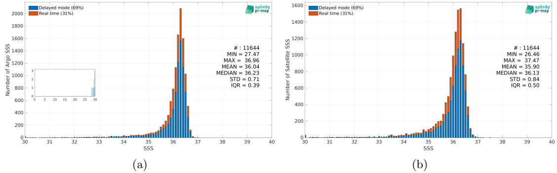
Figure 2: Histograms of SSS from Argo (a) and SMOS SSS L4 v1 - Weekly (CMEMS-CNR) (b) considering all match-up pairs per bins of 0.1 over the Gulf of Mexico Pi-MEP region and for the full satellite product period.
