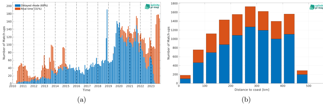
Figure 1: Number of match-ups between Argo and SMOS SSS L4 v1 - Weekly (CMEMS-CNR) SSS as a function of time (a) and as function of the distance to coast (b) over the Gulf of Mexico Pi-MEP region and for the full satellite product period.
