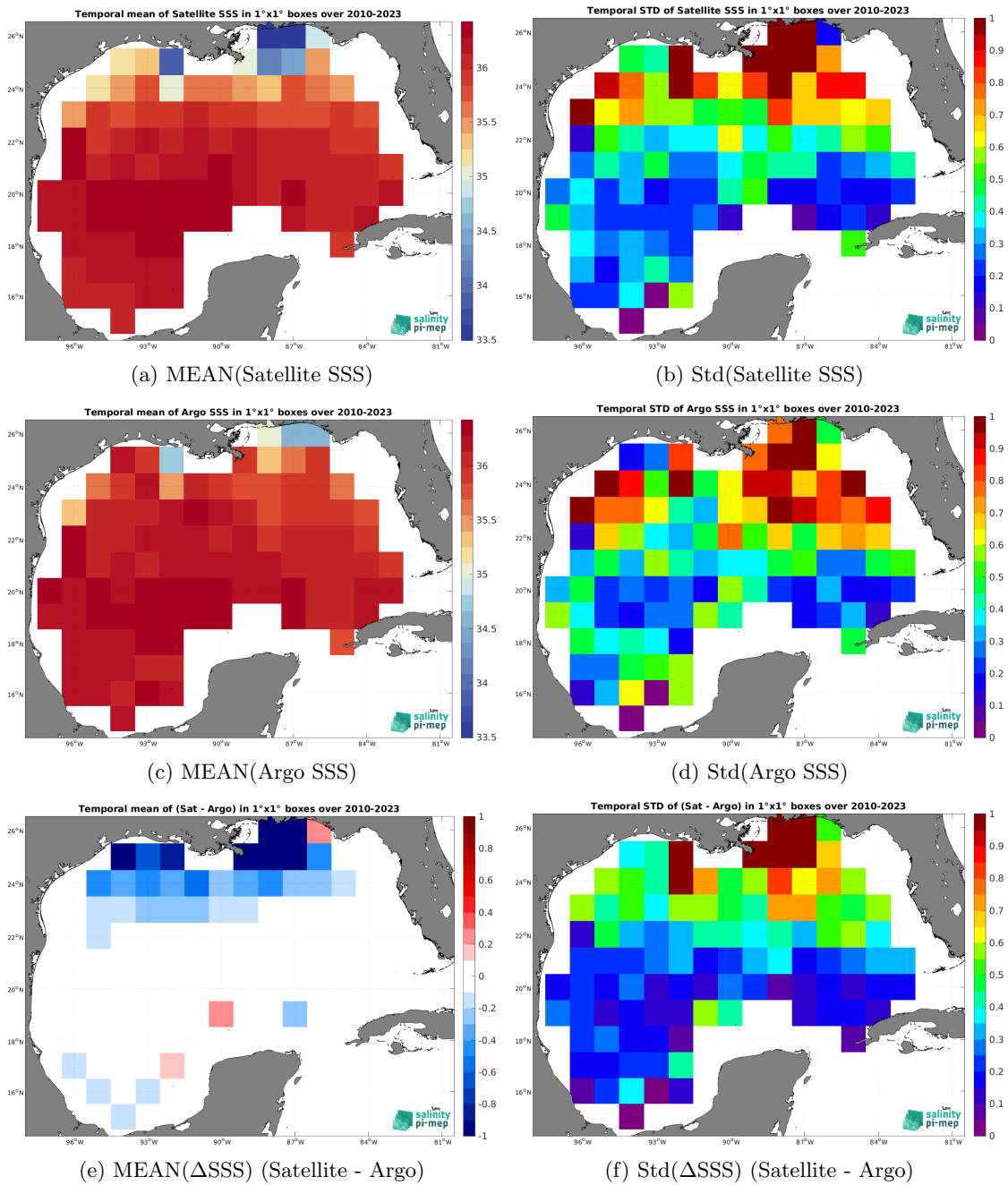
Figure 6: Temporal mean (left) and Std (right) of SSS from SMOS SSS L4 v1 - Weekly (CMEMS-CNR) (top), Argo (middle), and of \Delta SSS (Satellite - Argo). Only match-up pairs are used to generate these maps.
