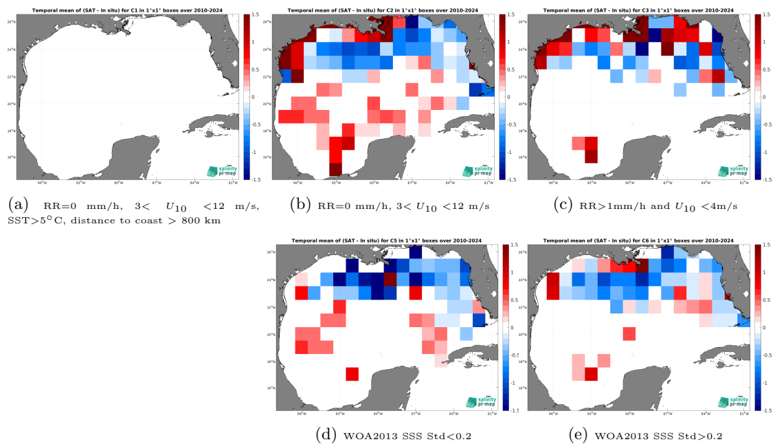
Figure 14: Temporal mean gridded over spatial boxes of size 1^\circ \times 1^\circ of \Delta\text{SSS} (SMOS SSS L4 v1 - Monthly (CMEMS-CNR) - TSG (SAMOS)) for 5 different subdatasets corresponding to:RR=0 mm/h, 3 < U_{10} < 12 m/s, SST > 5^\circ\text{C} , distance to coast > 800 km (a), RR=0 mm/h, 3 < U_{10} < 12 m/s (b), RR > 1 mm/h and U_{10} < 4 m/s (c), WOA2013 SSS Std < 0.2 (d), WOA2013 SSS Std > 0.2 (e).
