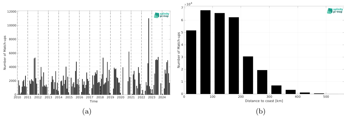
Figure 2: Number of match-ups between TSG (SAMOS) and SMOS SSS L4 v1 - Monthly (CMEMS-CNR) SSS as a function of time (a) and as function of the distance to coast (b) over the Gulf of Mexico Pi-MEP region and for the full satellite product period.
