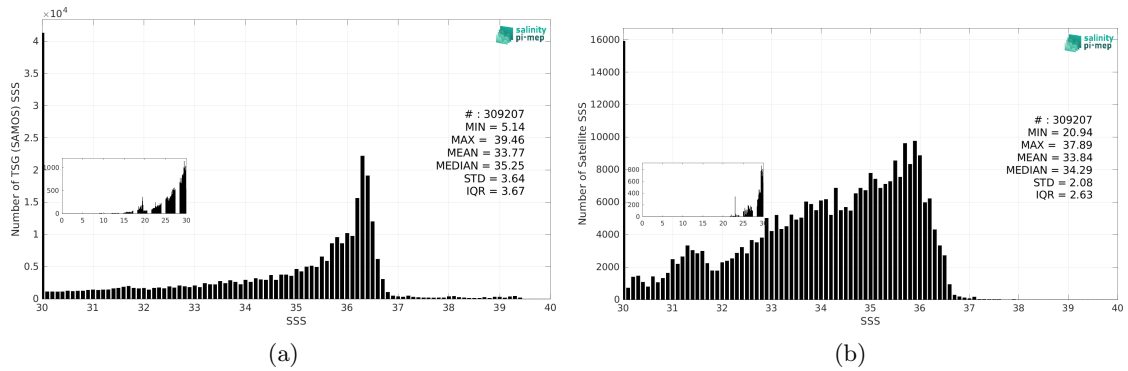
Figure 3: Histograms of SSS from TSG (SAMOS) (a) and SMOS SSS L4 v1 - Monthly (CMEMS-CNR) (b) considering all match-up pairs per bins of 0.1 over the Gulf of Mexico Pi-MEP region and for the full satellite product period.
