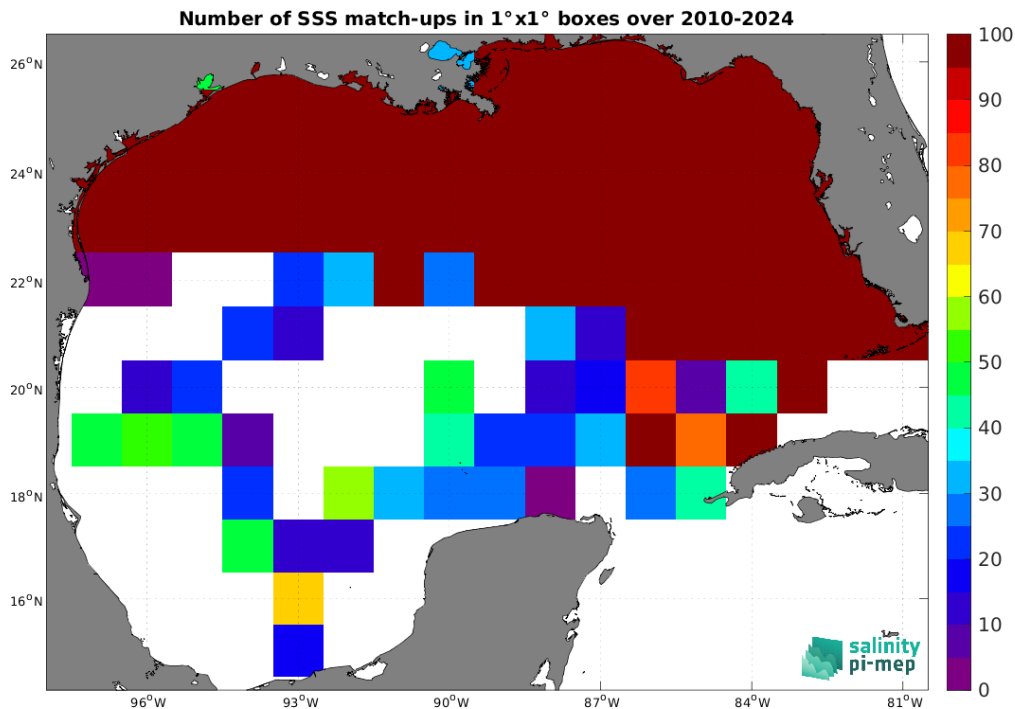
Figure 5: Number of SSS match-ups between TSG (SAMOS) SSS and the SMOS SSS L4 v1 - Monthly (CMEMS-CNR) SSS product for the Gulf of Mexico Pi-MEP region over 1^\circ \times 1^\circ boxes and for the full satellite product period.
