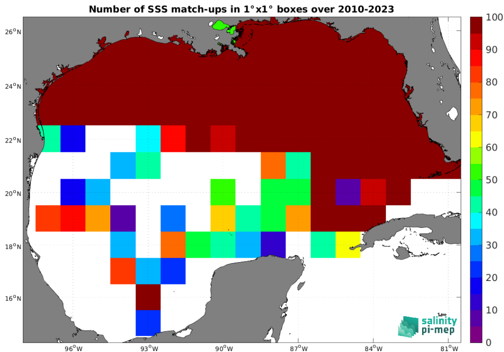
Figure 4: Number of SSS match-ups between TSG (SAMOS) SSS and the SMOS SSS L4 v1 - Monthly (CMEMS-CNR) SSS product for the Gulf of Mexico Pi-MEP region over 1^\circ \times 1^\circ boxes and for the full satellite product period.
