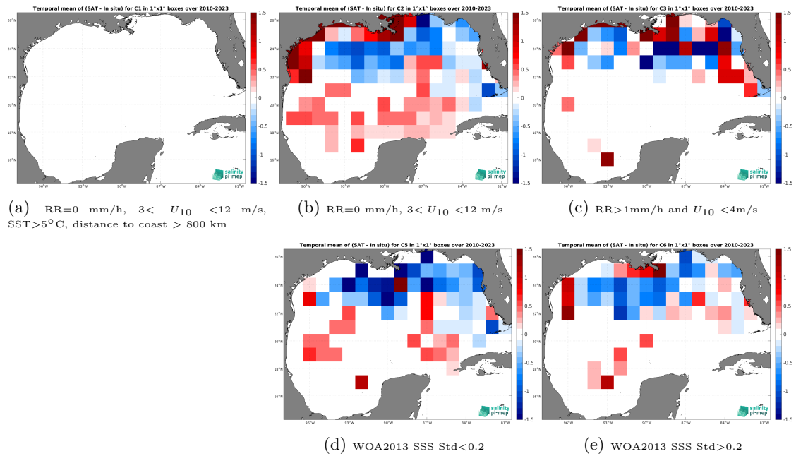
Figure 12: Temporal mean gridded over spatial boxes of size 1^\circ \times 1^\circ of \Delta\text{SSS} (SMOS SSS L4 v1 - Monthly (CMEMS-CNR) - TSG (SAMOS)) for 5 different subdatasets corresponding to:RR=0 mm/h, 3 < U_{10} < 12 m/s, SST > 5^\circ\text{C} , distance to coast > 800 km (a), RR=0 mm/h, 3 < U_{10} < 12 m/s (b), RR > 1 mm/h and U_{10} < 4 m/s (c), WOA2013 SSS Std < 0.2 (d), WOA2013 SSS Std > 0.2 (e).
