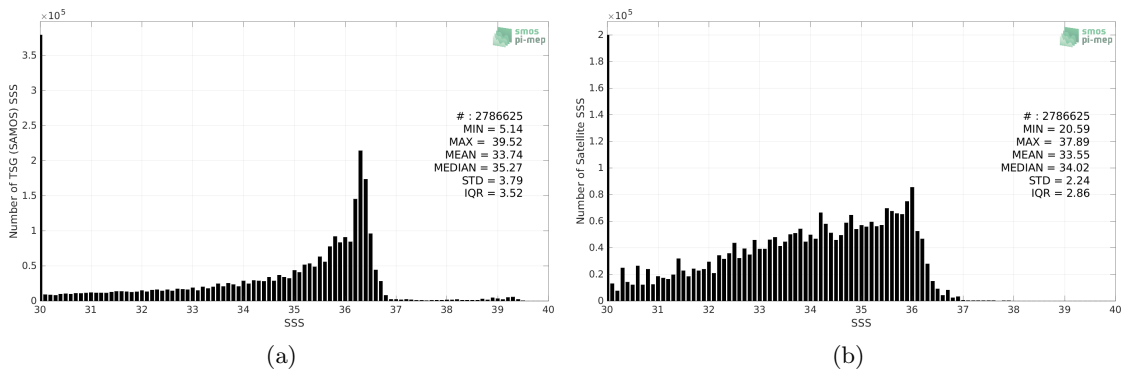
Figure 2: Histograms of SSS from TSG (SAMOS) (a) and SMOS SSS L4 v1 - Monthly (CMEMS-CNR) (b) considering all match-up pairs per bins of 0.1 over the Gulf of Mexico Pi-MEP region and for the full satellite product period.
