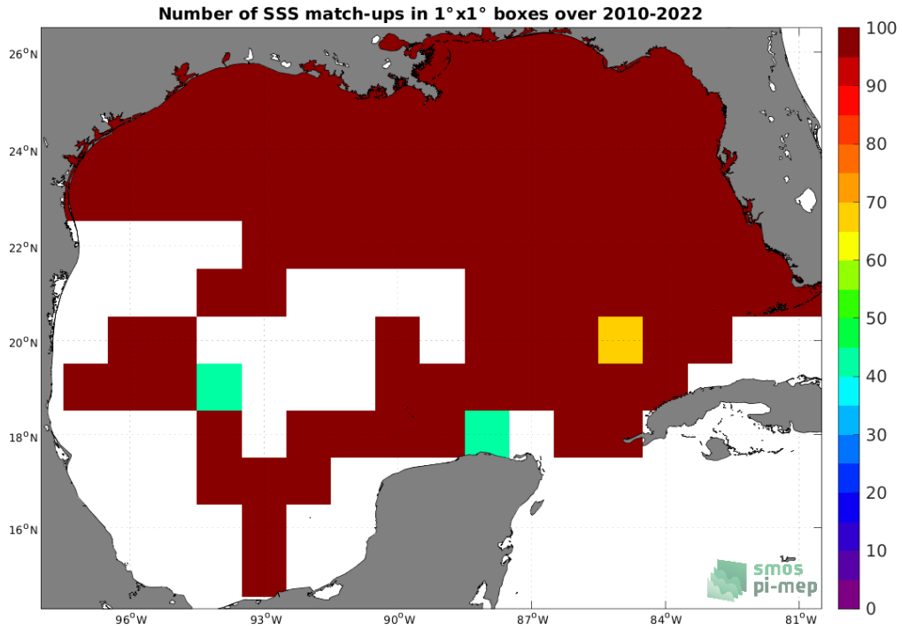
Figure 4: Number of SSS match-ups between TSG (SAMOS) SSS and the SMOS SSS L4 v1 - Monthly (CMEMS-CNR) SSS product for the Gulf of Mexico Pi-MEP region over 1°x1° boxes and for the full satellite product period.
