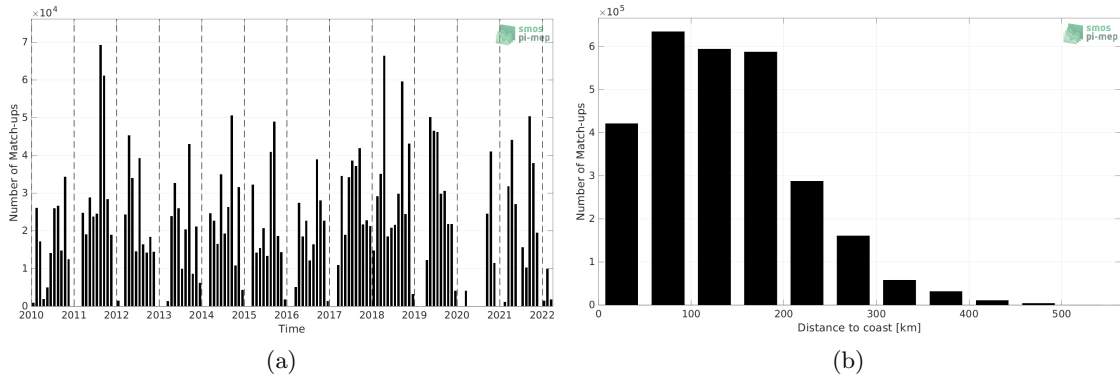
Figure 1: Number of match-ups between TSG (SAMOS) and SMOS SSS L4 v1 - Monthly (CMEMS-CNR) SSS as a function of time (a) and as function of the distance to coast (b) over the Gulf of Mexico Pi-MEP region and for the full satellite product period.
