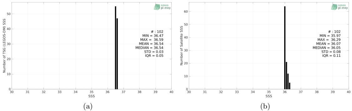
Figure 2: Histograms of SSS from TSG (LEGOS-DM) (a) and SMOS SSS L4 v1 - Monthly (CMEMS-CNR) (b) considering all match-up pairs per bins of 0.1 over the Gulf of Mexico Pi-MEP region and for the full satellite product period.
