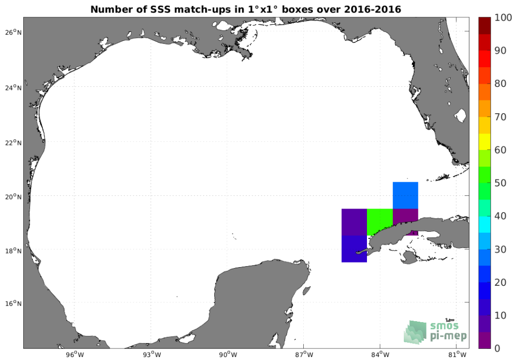
Figure 4: Number of SSS match-ups between TSG (LEGOS-DM) SSS and the SMOS SSS L4 v1 - Monthly (CMEMS-CNR) SSS product for the Gulf of Mexico Pi-MEP region over 1^\circ \times 1^\circ boxes and for the full satellite product period.
