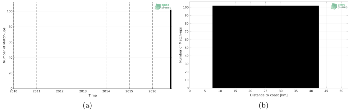
Figure 1: Number of match-ups between TSG (LEGOS-DM) and SMOS SSS L4 v1 - Monthly (CMEMS-CNR) SSS as a function of time (a) and as function of the distance to coast (b) over the Gulf of Mexico Pi-MEP region and for the full satellite product period.
