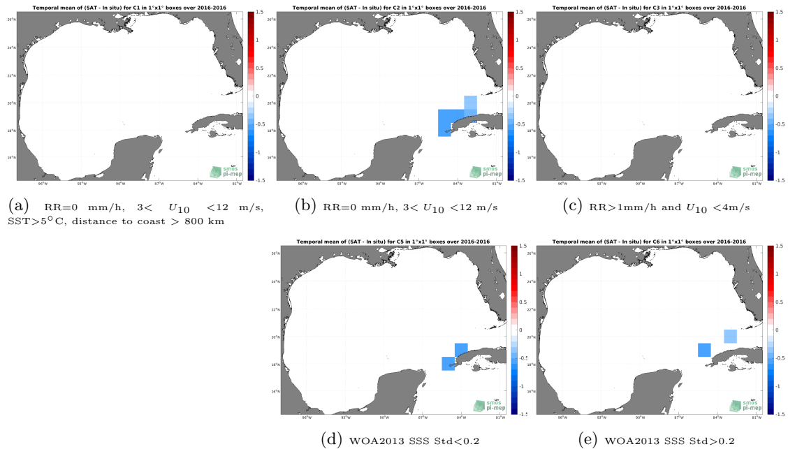
Figure 12: Temporal mean gridded over spatial boxes of size 1^{\circ}\times 1^{\circ} of \Delta\text{SSS} (SMOS SSS L4 v1 - Monthly (CMEMS-CNR) - TSG (LEGOS-DM)) for 5 different subdatasets corresponding to:RR=0 mm/h, 3 < U_{10} < 12 m/s, SST >5^{\circ}\text{C} , distance to coast > 800 km (a), RR=0 mm/h, 3 < U_{10} < 12 m/s (b), RR >1 mm/h and U_{10} < 4 m/s (c), WOA2013 SSS Std <0.2 (d), WOA2013 SSS Std >0.2 (e).
