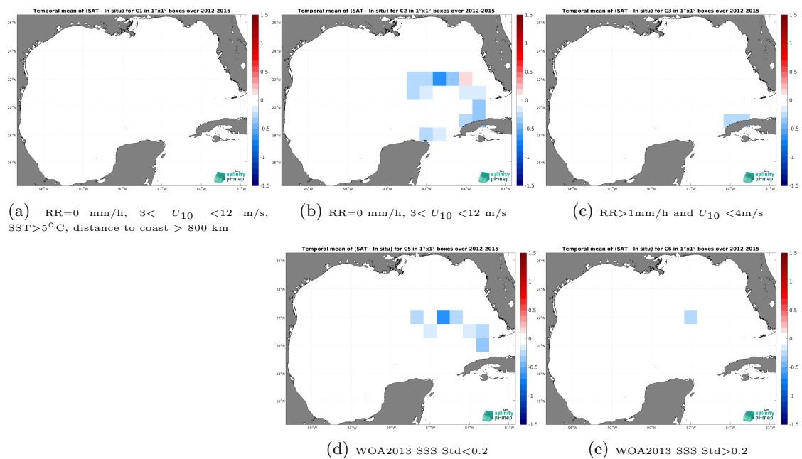
Figure 14: Temporal mean gridded over spatial boxes of size 1^\circ \times 1^\circ of \Delta SSS (SMOS SSS L4 v1 - Monthly (CMEMS-CNR) - TSG (GOSUD-Sailing-ship)) for 5 different subdatasets corresponding to:RR=0 mm/h, 3 < U_{10} < 12 m/s, SST >5^\circ C, distance to coast > 800 km (a), RR=0 mm/h, 3 < U_{10} < 12 m/s (b), RR >1 mm/h and U_{10} < 4 m/s (c), WOA2013 SSS Std <0.2 (d), WOA2013 SSS Std >0.2 (e).
