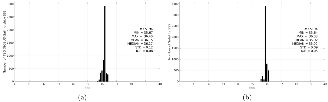
Figure 3: Histograms of SSS from TSG (GOSUD-Sailing-ship) (a) and SMOS SSS L4 v1 - Monthly (CMEMS-CNR) (b) considering all match-up pairs per bins of 0.1 over the Gulf of Mexico Pi-MEP region and for the full satellite product period.
