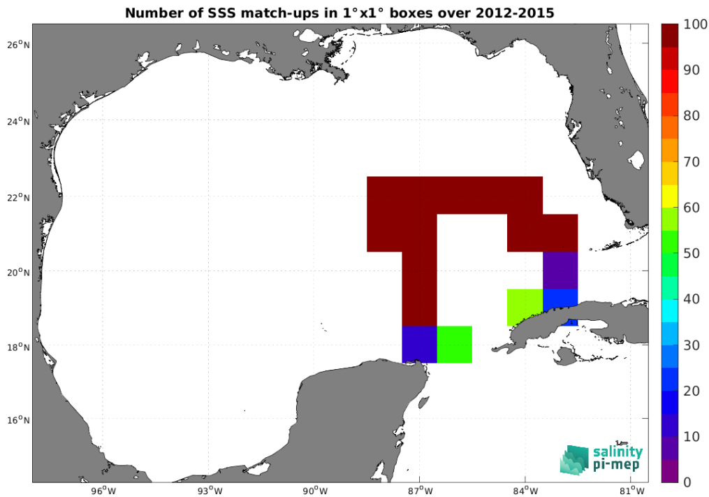
Figure 5: Number of SSS match-ups between TSG (GOSUD-Sailing-ship) SSS and the SMOS SSS L4 v1 - Monthly (CMEMS-CNR) SSS product for the Gulf of Mexico Pi-MEP region over 1°×1° boxes and for the full satellite product period.
