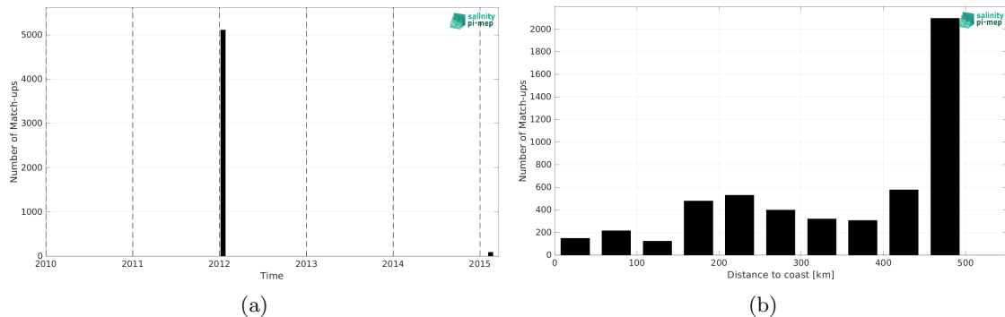
Figure 2: Number of match-ups between TSG (GOSUD-Sailing-ship) and SMOS SSS L4 v1 - Monthly (CMEMS-CNR) SSS as a function of time (a) and as function of the distance to coast (b) over the Gulf of Mexico Pi-MEP region and for the full satellite product period.
