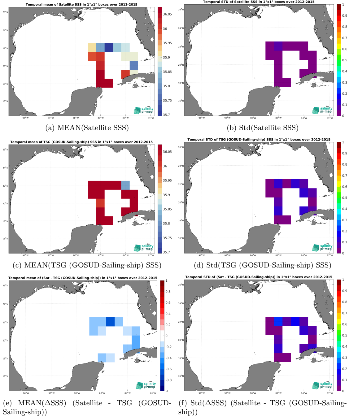
Figure 7: Temporal mean (left) and Std (right) of SSS from SMOS SSS L4 v1 - Monthly (CMEMS-CNR) (top), TSG (GOSUD-Sailing-ship) (middle), and of \Delta SSS (Satellite - TSG (GOSUD-Sailing-ship)). Only match-up pairs are used to generate these maps.
