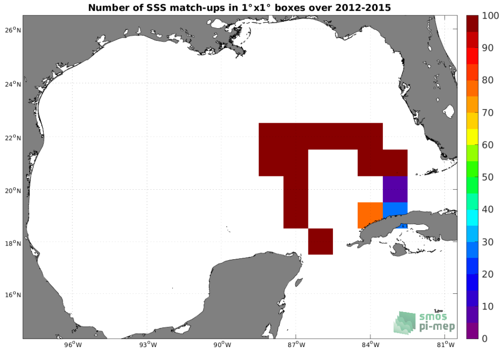
Figure 4: Number of SSS match-ups between TSG (GOSUD-Sailing-ship) SSS and the SMOS SSS L4 v1 - Monthly (CMEMS-CNR) SSS product for the Gulf of Mexico Pi-MEP region over 1^\circ \times 1^\circ boxes and for the full satellite product period.
