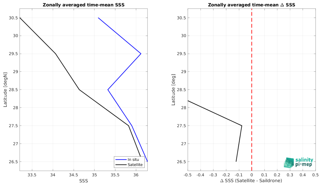
Figure 9: Left panel: Zonal mean SSS from SMOS SSS L4 v1 - Monthly (CMEMS-CNR) satellite product (black) and from Sairdrone (blue). Right panel: Zonal mean of \Delta SSS (Satellite - Sairdrone) for all the collected Pi-MEP match-up pairs estimated over the full satellite product period.
