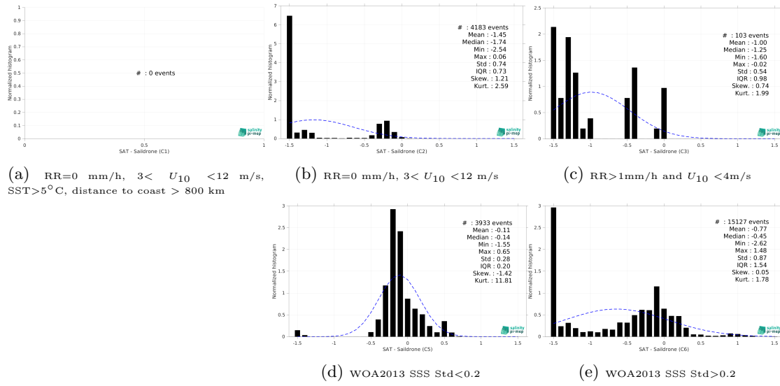
Figure 15: Normalized histogram of \Delta\text{SSS} (SMOS SSS L4 v1 - Monthly (CMEMS-CNR) - Saildrone) for 5 different subdatasets corresponding to: RR=0 mm/h, 3 < U_{10} < 12 m/s, SST > 5^{\circ}\text{C} , distance to coast > 800 km (a), RR=0 mm/h, 3 < U_{10} < 12 m/s (b), RR > 1\text{mm/h} and U_{10} < 4\text{m/s} (c), WOA2013 SSS Std < 0.2 (d), WOA2013 SSS Std > 0.2 (e).
