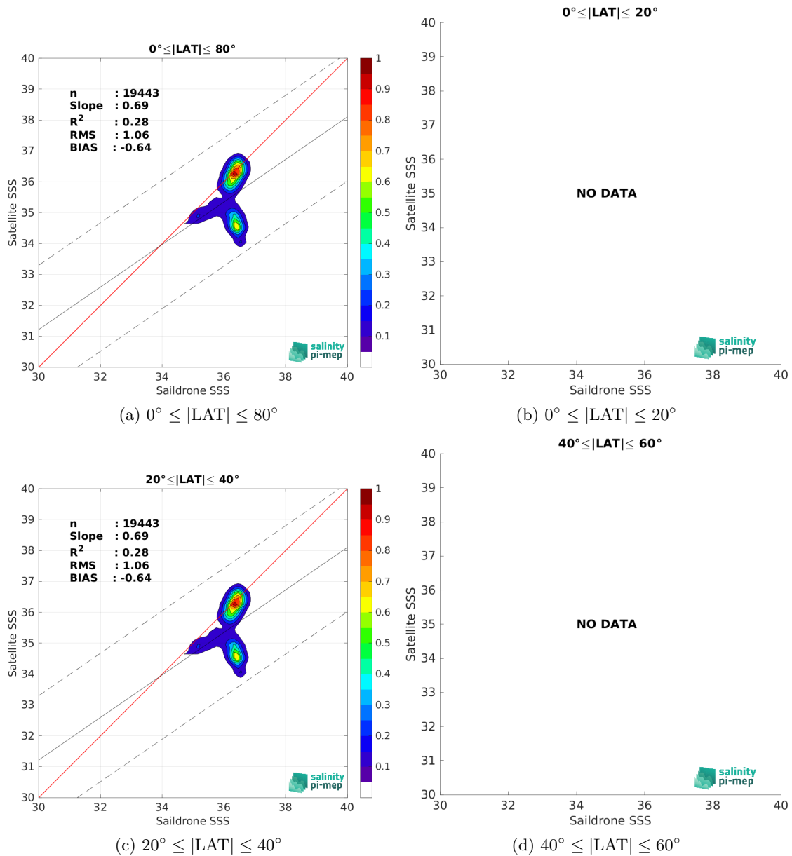
Figure 10: Contour maps of the concentration of SMOS SSS L4 v1 - Monthly (CMEMS-CNR) SSS (y-axis) versus Saildrone SSS (x-axis) at match-up pairs for different latitude bands. For each plot, the red line shows x=y . The black thin and dashed lines indicate a linear fit through the data cloud and the \pm 95\% confidence levels, respectively. The number match-up pairs n , the slope and R^2 coefficient of the linear fit, the root mean square (RMS) and the mean bias between satellite and in situ data are indicated for each latitude band in each plots.
