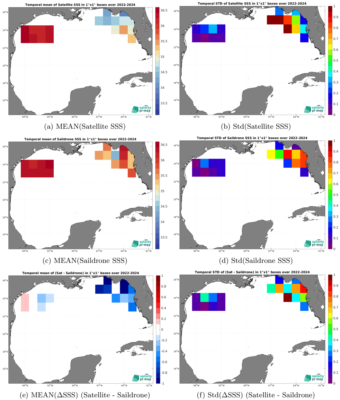
Figure 7: Temporal mean (left) and Std (right) of SSS from SMOS SSS L4 v1 - Monthly (CMEMS-CNR) (top), Saildrone (middle), and of \Delta SSS (Satellite - Saildrone). Only match-up pairs are used to generate these maps.
