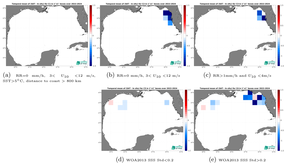
Figure 14: Temporal mean gridded over spatial boxes of size 1^\circ \times 1^\circ of \Delta SSS (SMOS SSS L4 v1 - Monthly (CMEMS-CNR) - Saildrone) for 5 different subdatasets corresponding to:RR=0 mm/h, 3 < U_{10} < 12 m/s, SST >5^\circ C, distance to coast > 800 km (a), RR=0 mm/h, 3 < U_{10} < 12 m/s (b), RR >1 mm/h and U_{10} < 4 m/s (c), WOA2013 SSS Std <0.2 (d), WOA2013 SSS Std >0.2 (e).
