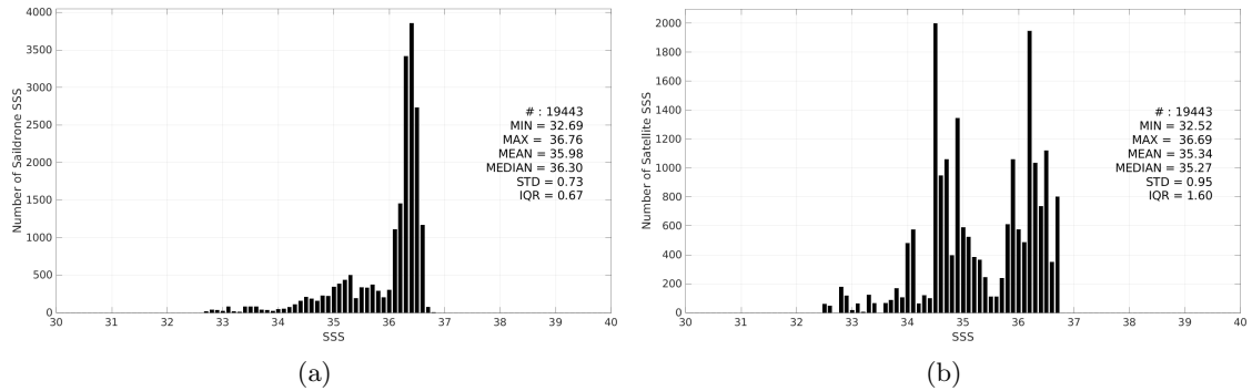
Figure 3: Histograms of SSS from Saildrone (a) and SMOS SSS L4 v1 - Monthly (CMEMS-CNR) (b) considering all match-up pairs per bins of 0.1 over the Gulf of Mexico Pi-MEP region and for the full satellite product period.
