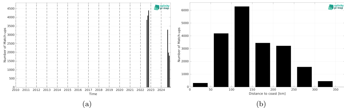
Figure 2: Number of match-ups between Saildrone and SMOS SSS L4 v1 - Monthly (CMEMS-CNR) SSS as a function of time (a) and as function of the distance to coast (b) over the Gulf of Mexico Pi-MEP region and for the full satellite product period.
