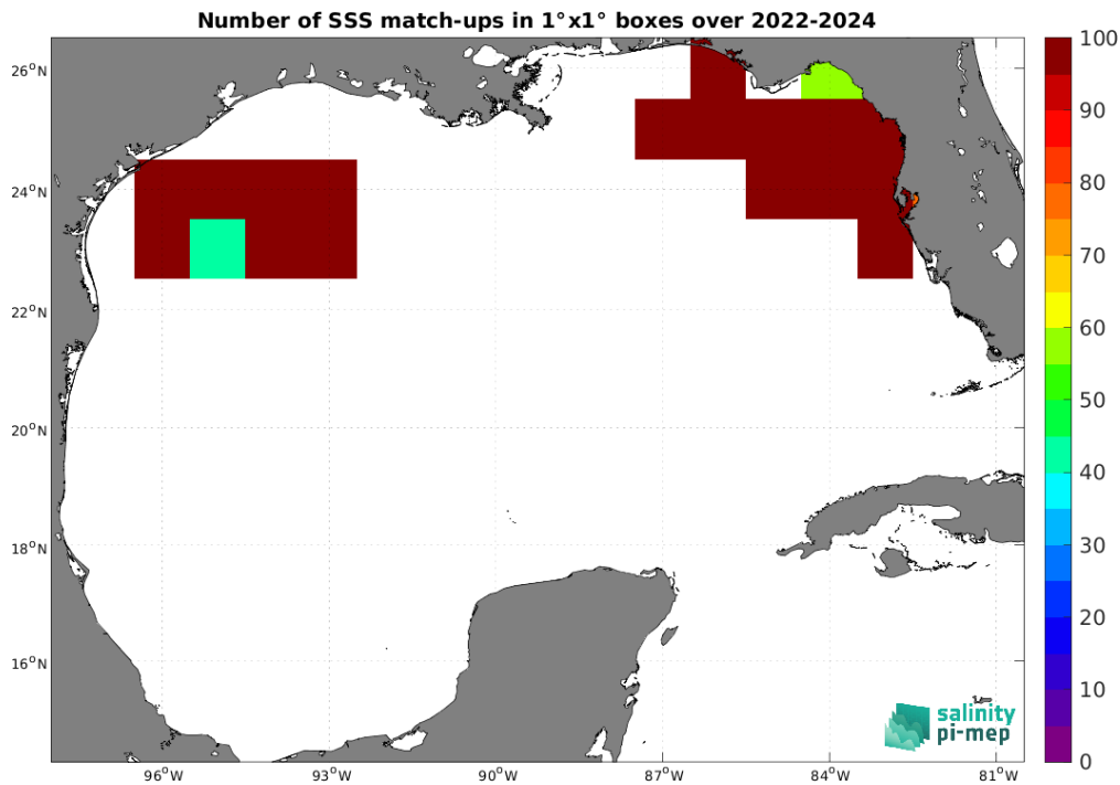
Figure 5: Number of SSS match-ups between Saildrone SSS and the SMOS SSS L4 v1 - Monthly (CMEMS-CNR) SSS product for the Gulf of Mexico Pi-MEP region over 1^\circ \times 1^\circ boxes and for the full satellite product period.
