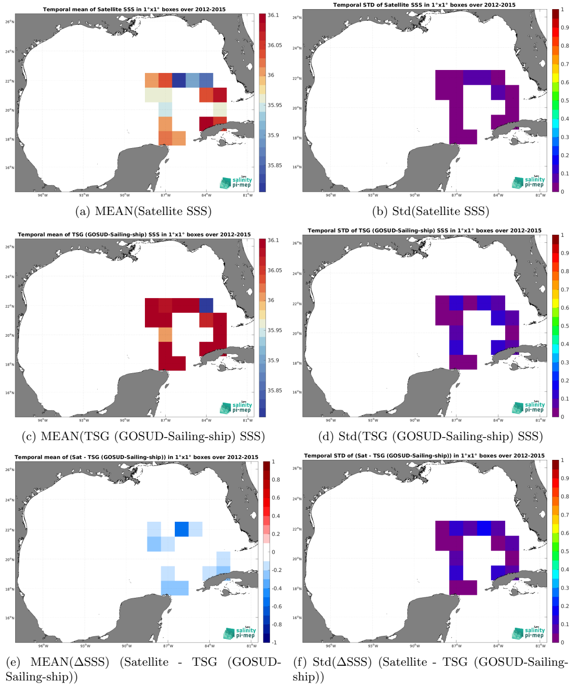
Figure 7: Temporal mean (left) and Std (right) of SSS from SMOS SSS L4 v1 - Daily (CMEMS-CNR) (top), TSG (GOSUD-Sailing-ship) (middle), and of \Delta SSS (Satellite - TSG (GOSUD-Sailing-ship)). Only match-up pairs are used to generate these maps.
