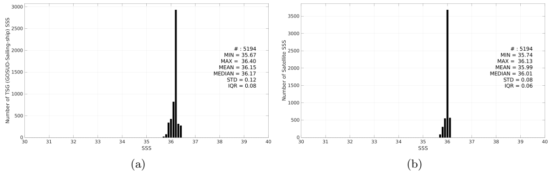
Figure 3: Histograms of SSS from TSG (GOSUD-Sailing-ship) (a) and SMOS SSS L4 v1 - Daily (CMEMS-CNR) (b) considering all match-up pairs per bins of 0.1 over the Gulf of Mexico Pi-MEP region and for the full satellite product period.
