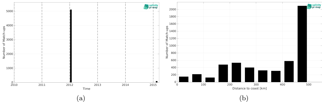
Figure 2: Number of match-ups between TSG (GOSUD-Sailing-ship) and SMOS SSS L4 v1 - Daily (CMEMS-CNR) SSS as a function of time (a) and as function of the distance to coast (b) over the Gulf of Mexico Pi-MEP region and for the full satellite product period.
