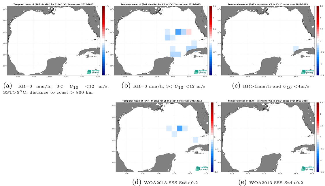
Figure 14: Temporal mean gridded over spatial boxes of size 1^\circ \times 1^\circ of \Delta SSS (SMOS SSS L4 v1 - Daily (CMEMS-CNR) - TSG (GOSUD-Sailing-ship)) for 5 different subdatasets corresponding to:RR=0 mm/h, 3 < U_{10} < 12 m/s, SST >5^\circ C, distance to coast > 800 km (a), RR=0 mm/h, 3 < U_{10} < 12 m/s (b), RR >1 mm/h and U_{10} < 4 m/s (c), WOA2013 SSS Std <0.2 (d), WOA2013 SSS Std >0.2 (e).
