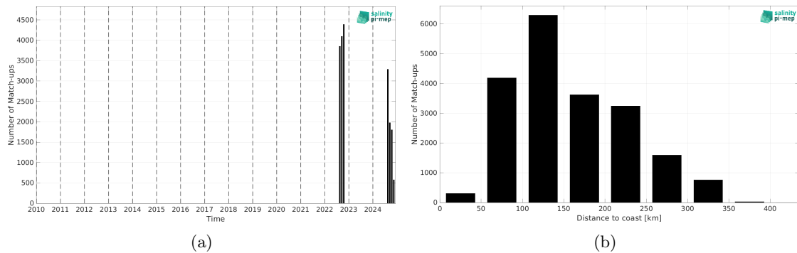
Figure 2: Number of match-ups between Saildrone and SMOS SSS L4 v1 - Daily (CMEMS-CNR) SSS as a function of time (a) and as function of the distance to coast (b) over the Gulf of Mexico Pi-MEP region and for the full satellite product period.
