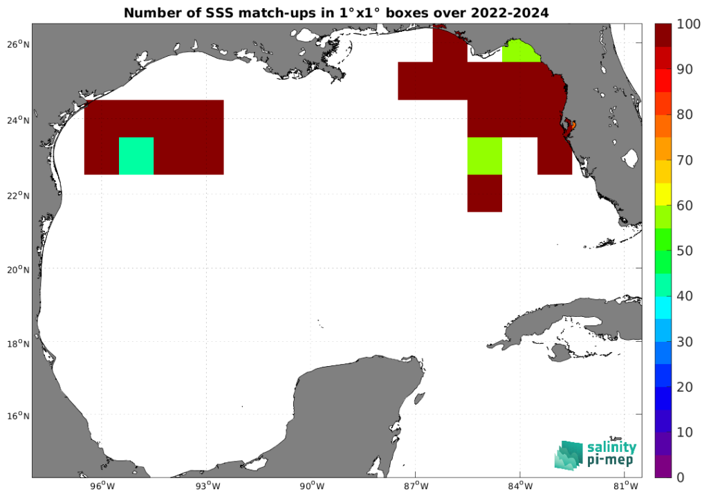
Figure 5: Number of SSS match-ups between Saildrone SSS and the SMOS SSS L4 v1 - Daily (CMEMS-CNR) SSS product for the Gulf of Mexico Pi-MEP region over 1^\circ \times 1^\circ boxes and for the full satellite product period.
