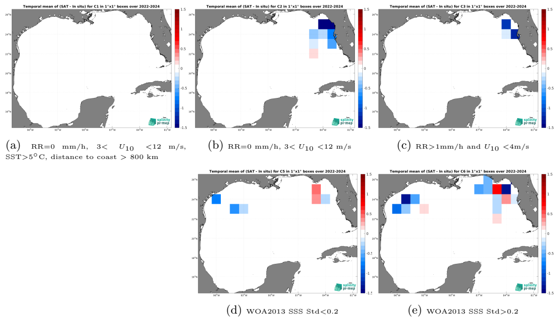
Figure 14: Temporal mean gridded over spatial boxes of size 1^\circ \times 1^\circ of \Delta SSS (SMOS SSS L4 v1 - Daily (CMEMS-CNR) - Saildrone) for 5 different subdatasets corresponding to:RR=0 mm/h, 3 < U_{10} < 12 m/s, SST >5^\circ\text{C} , distance to coast > 800 km (a), RR=0 mm/h, 3 < U_{10} < 12 m/s (b), RR >1 mm/h and U_{10} < 4 m/s (c), WOA2013 SSS Std <0.2 (d), WOA2013 SSS Std >0.2 (e).
