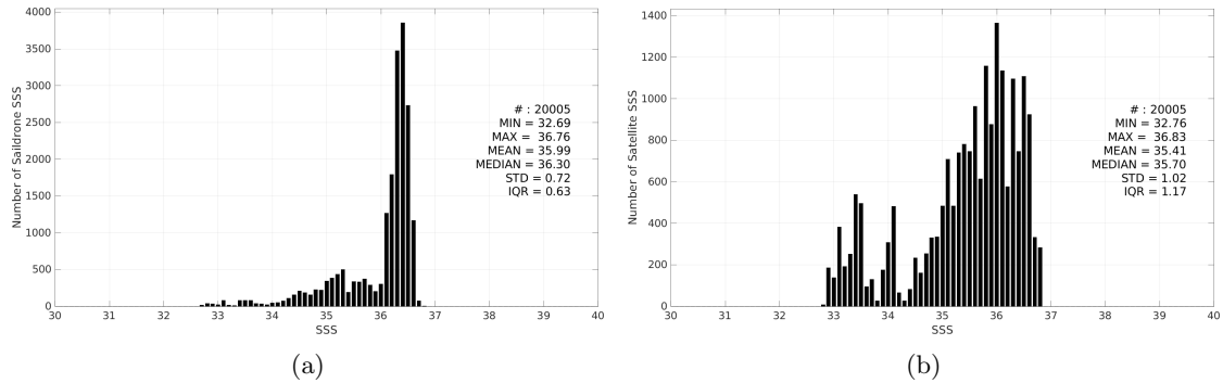
Figure 3: Histograms of SSS from Saildrone (a) and SMOS SSS L4 v1 - Daily (CMEMS-CNR) (b) considering all match-up pairs per bins of 0.1 over the Gulf of Mexico Pi-MEP region and for the full satellite product period.
