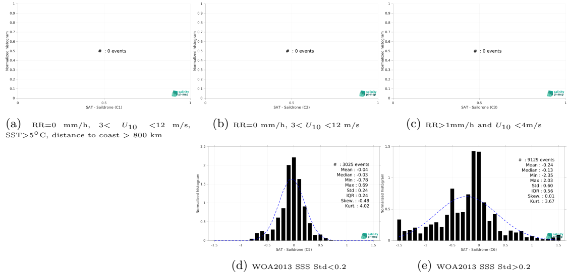
Figure 15: Normalized histogram of \Delta SSS (SMOS SSS L4 v1 - Daily (CMEMS-CNR) - Sairdrone) for 5 different subdatasets corresponding to: RR=0 mm/h, 3 < U_{10} < 12 m/s, SST >5^{\circ} C, distance to coast > 800 km (a), RR=0 mm/h, 3 < U_{10} < 12 m/s (b), RR >1 mm/h and U_{10} < 4 m/s (c), WOA2013 SSS Std <0.2 (d), WOA2013 SSS Std >0.2 (e).
